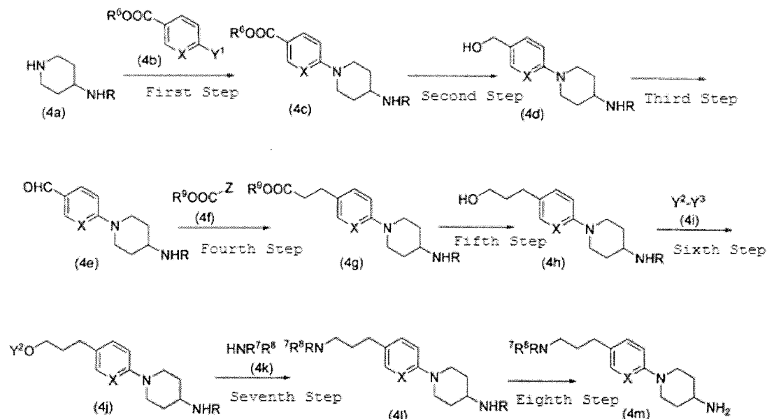
Reaction Scheme 4
