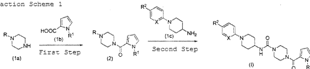
Reaction Scheme 1
