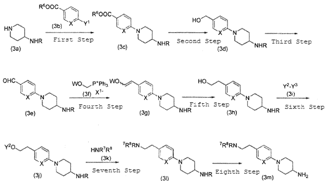
Reaction Scheme 3
