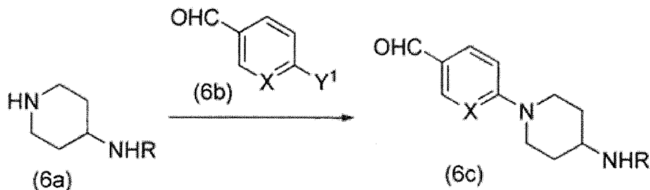
Reaction Scheme 6
