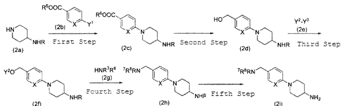
Reaction Scheme 2
