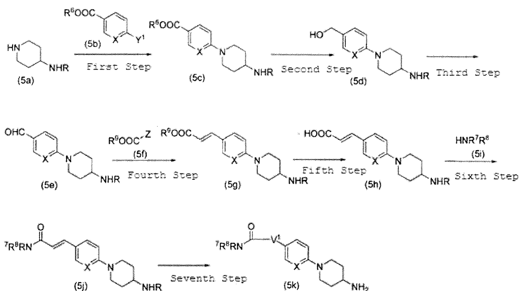
Reaction Scheme 5
