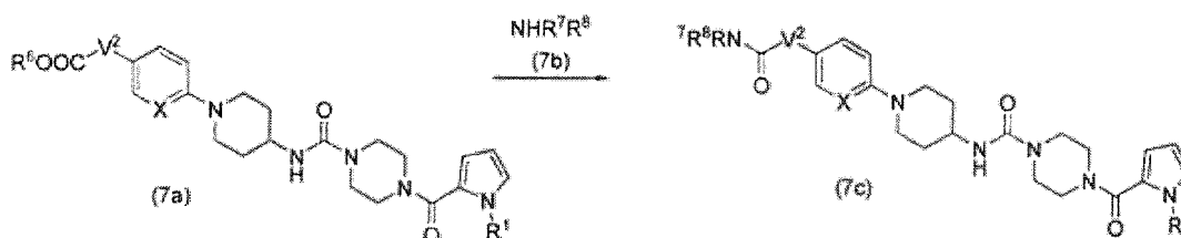
Reaction Scheme 7
