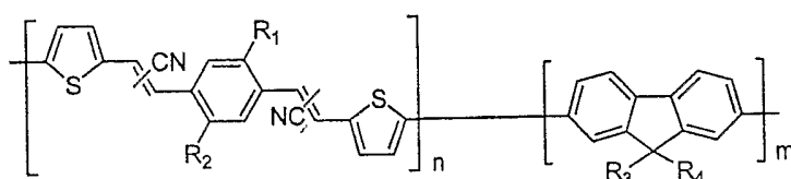
Formula 1
