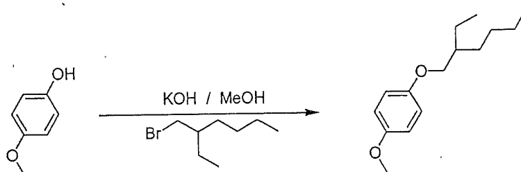
Reaction Scheme 1
