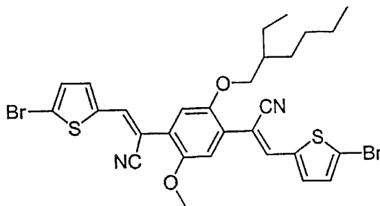
Formula 4
