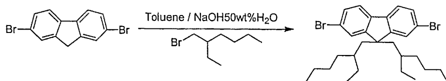
Reaction Scheme 5
