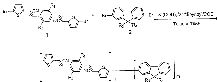
Reaction Scheme 6
