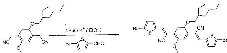
Reaction Scheme 4
