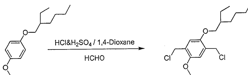
Reaction Scheme 2
