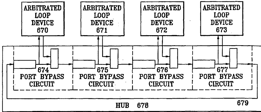
Fig. 22 (PRIOR ART)
