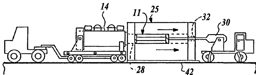
Fig. 4. (PRIOR ART)
