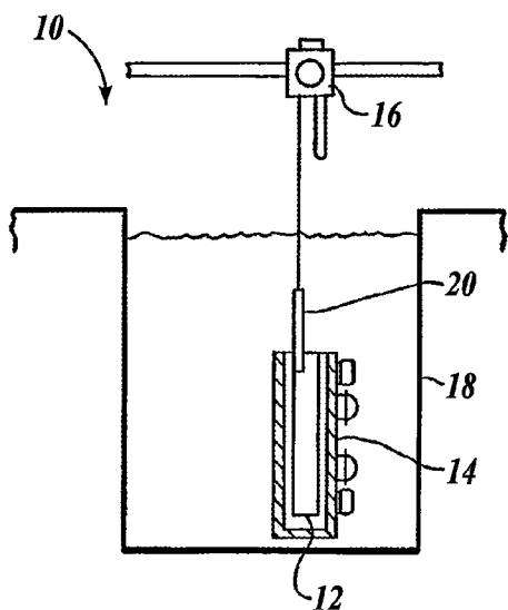
Fig. 1. (PRIOR ART)
