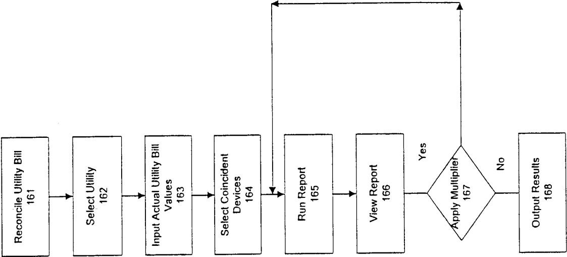
Figure 9: Reconcile Utility Bill Flowchart
