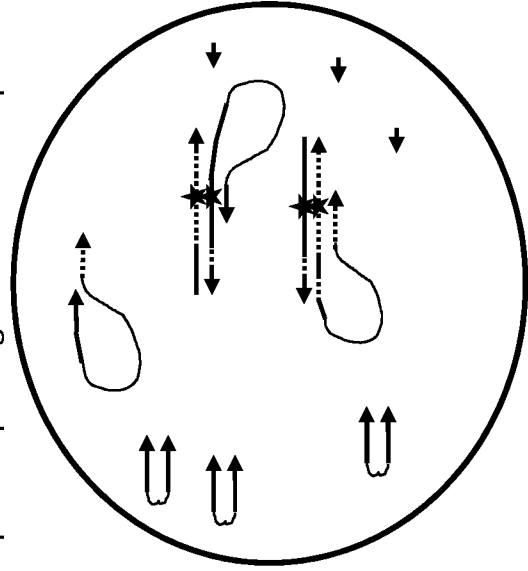
Step 3: Displacing extension of captured targets only
