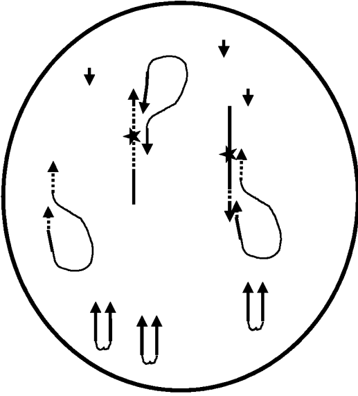
Step 2: Universal primer binds only to captured targets
