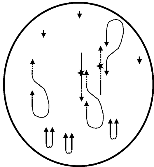
Step 1: Denature and Target Capture
