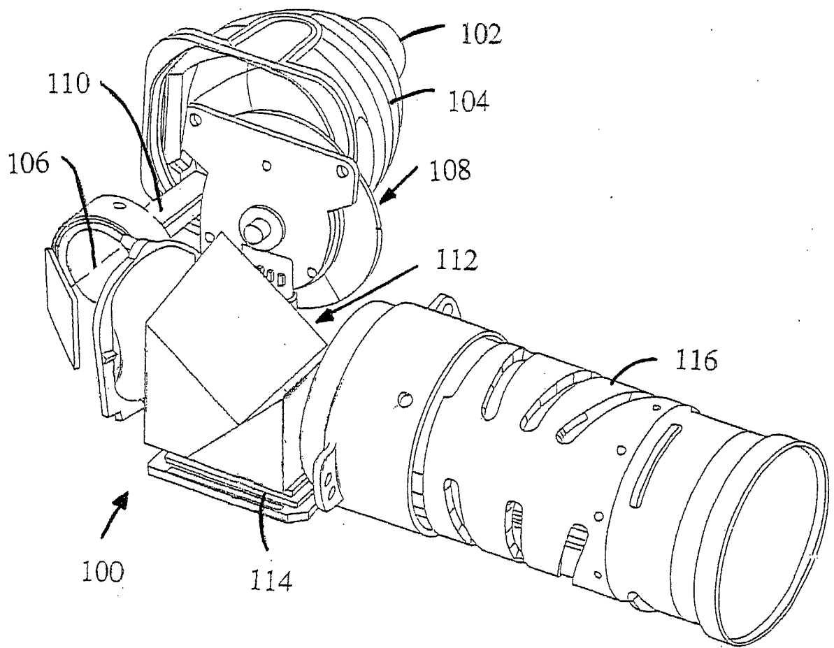
Fig. 1 (Prior Art)
