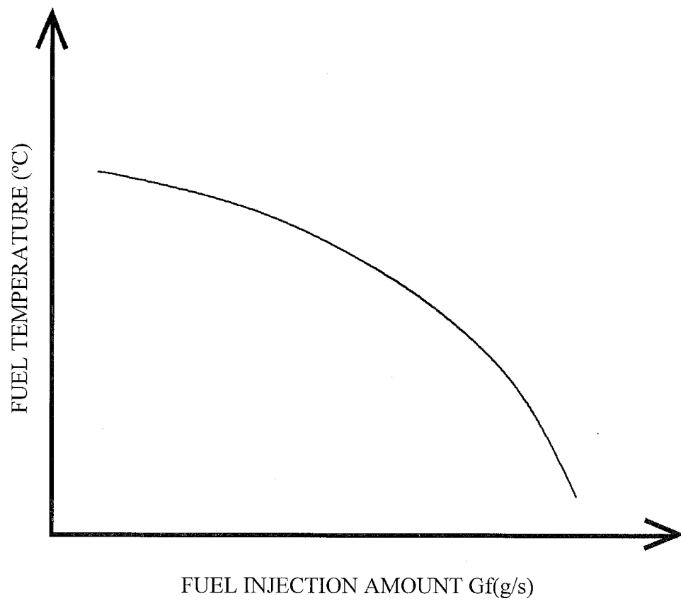
MAP FOR CALCULATING FUEL TEMPERATURE
