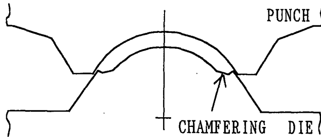
FIG. 16 (C) CURVING
