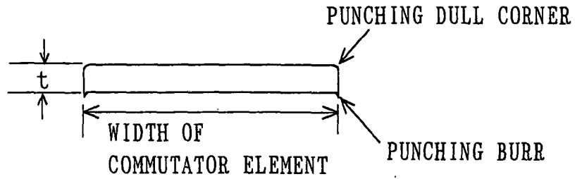
FIG. 16 (B) CHAMFERING
