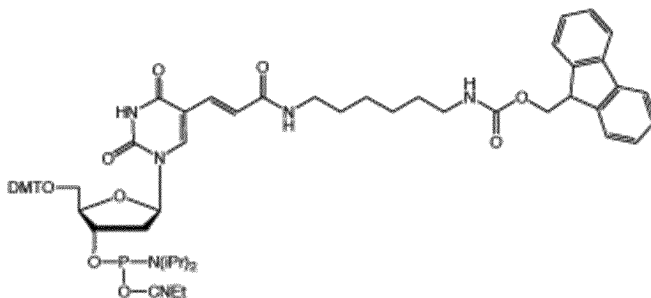
[0194] S-Bz-thiol-modifier C6-dT .
