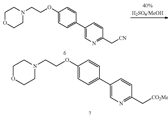
Preparation of methyl 2-(5-(4-(2-morpholinoethoxy)phenyl)pyridin-2-yl)acetate (7)
