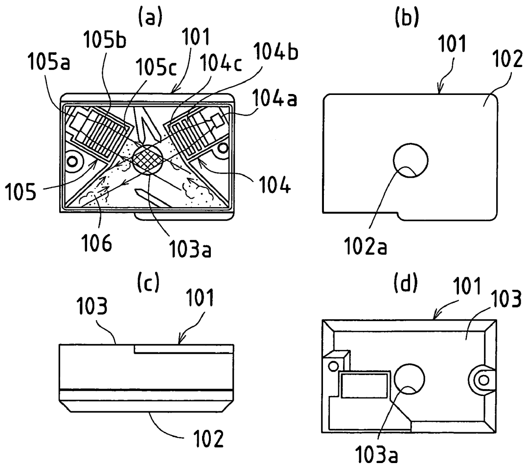
FIG. 6 Prior Art
