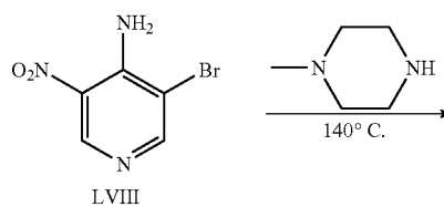
Scheme 13
