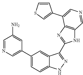
5-(3-(7-(Thiophen-3-yl)-3H-imidazo[4,5-c]pyridin-2-yl)-1H-indazol-5-yl)pyridin-3-amine 291
