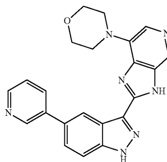
4-(2-(5-(pyridin-3-yl)-1H-indazol-3-yl)-3H-imidazo[4,5-c]pyridin-7-yl)morpholine 6
