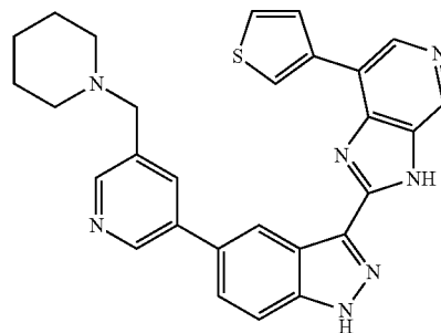
2-(5-(5-(Piperidin-1-ylmethyl)pyridin-3-yl)-1H-indazol-3-yl)-7-(thiophen-3-yl)-3H-imidazo[4,5-c]pyridine 303
