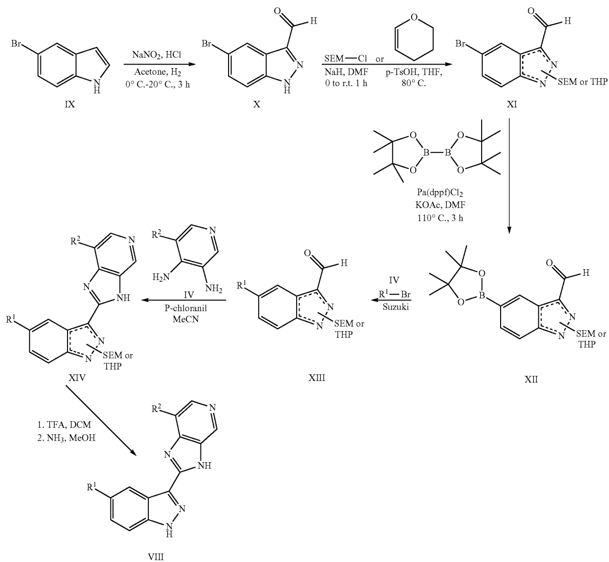
Scheme 2
