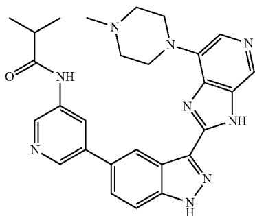
N-(5-(3-(7-(4-methylpiperazin-1-yl)-3H-imidazo[4,5-c]pyridin-2-yl)-1H-indazol-5-yl)pyridin-3-yl)isobutyramide 2
