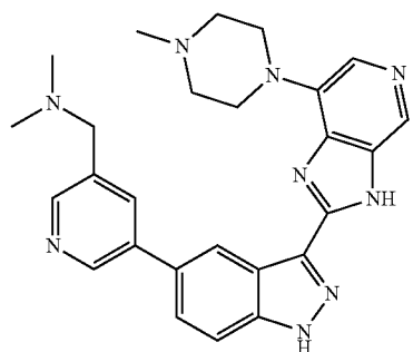
N,N-dimethyl-1-(5-(3-(7-(4-methylpiperazin-1-yl)-3H-imidazo[4,5-c]pyridin-2-yl)-1H-indazol-5-yl)pyridin-3-yl)methanamine 3
