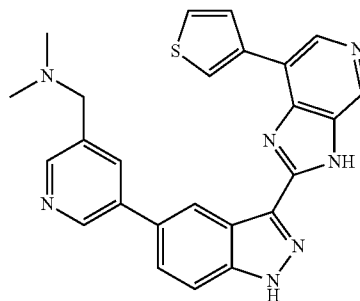
N,N-Dimethyl-1-(5-(3-(7-(thiophen-3-yl)-3H-imidazo[4,5-c]pyridin-2-yl)-1H-indazol-5-yl)pyridin-3-yl)methanamine 301
