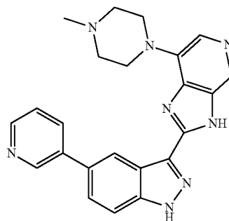
7-(4-methylpiperazin-1-yl)-2-(5-(pyridin-3-yl)-1H-indazol-3-yl)-3H-imidazo[4,5-c]pyridine 4
