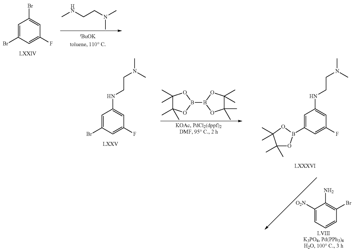
Scheme 14
