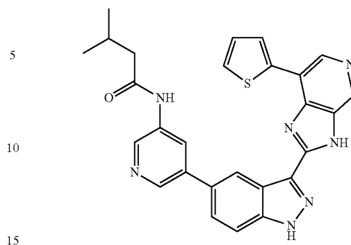
3-Methyl-N-(5-(3-(7-(thiophen-2-yl)-3H-imidazo[4,5-c]pyridin-2-yl)-1H-indazol-5-yl)pyridin-3-yl)butanamide 397
