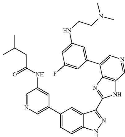
N-(5-(3-(7-(3-(2-(Dimethylamino)ethylamino)-5-fluorophenyl)-3H-imidazo[4,5-c]pyridin-2-yl)-1H-indazol-5-yl)pyridin-3-yl)-3-methylbutanamide 349
