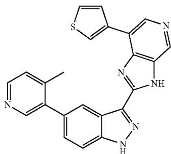
2-(5-(4-Methylpyridin-3-yl)-1H-indazol-3-yl)-7-(thiophen-3-yl)-3H-imidazo[4,5-c]pyridine 293
