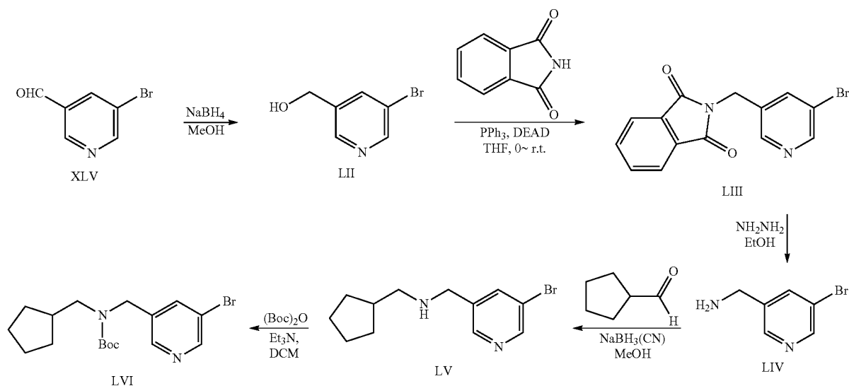
Scheme 11
