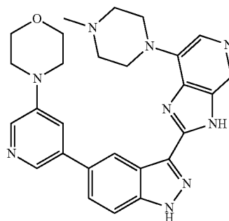
4-(5-(3-(7-(4-methylpiperazin-1-yl)-3H-imidazo[4,5-c]pyridin-2-yl)-1H-indazol-5-yl)pyridin-3-yl)morpholine 5
