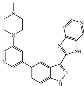
2-(5-(5-(4-methylpiperazin-1-yl)pyridin-3-yl)-1H-indazol-3-yl)-3H-imidazo[4,5-c]pyridine 7
