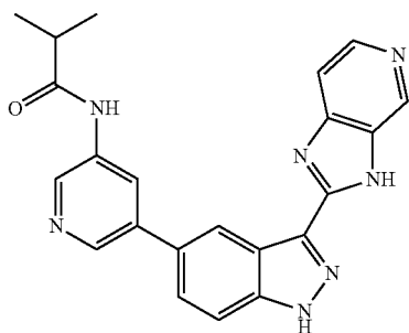
N-(5-(3-(3H-imidazo[4,5-c]pyridin-2-yl)-1H-indazol-5-yl)pyridin-3-yl)isobutyramide 9
