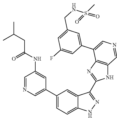
N-(5-(3-(7-(3-Fluoro-5-(methylsulfonamidomethyl)phenyl)-3H-imidazo[4,5-c]pyridin-2-yl)-1H-indazol-5-yl)pyridin-3-yl)-3-methylbutanamide 373
