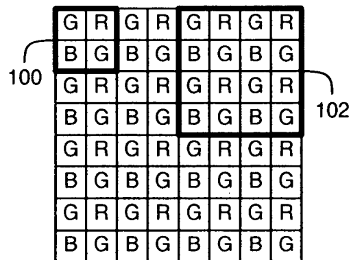
FIG. 2 (PRIOR ART)
