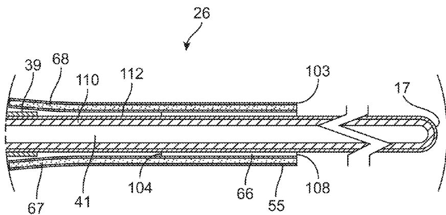
SECTION B-B ROTATED 90°
