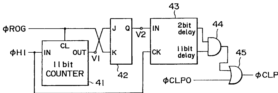
BLOCK DIAGRAM OF A TYPICAL CLAMP PULSE GENERATING CIRCUIT IMPLEMENTED BY THE FIRST EMBODIMENT
