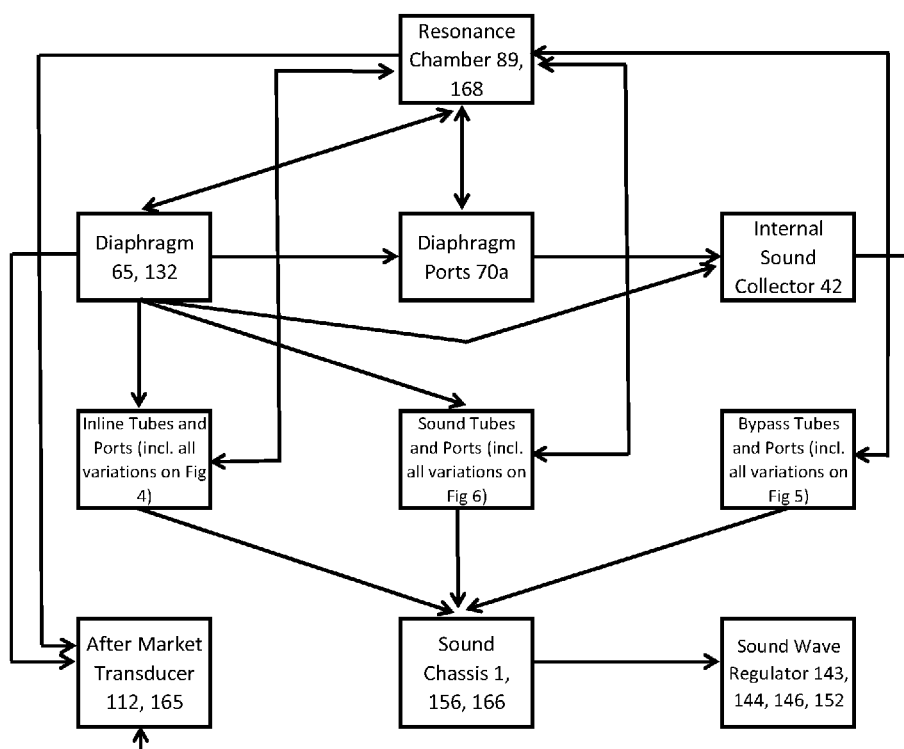
FIG. 28 Acoustic Soundwave Output System Pathway
