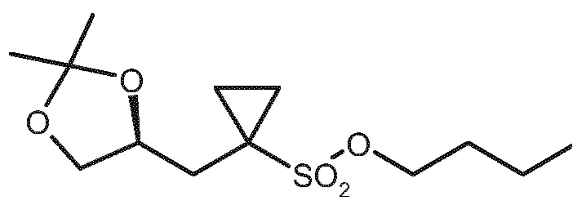
(S)-6
