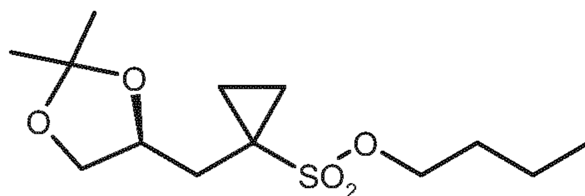
(S)-6
