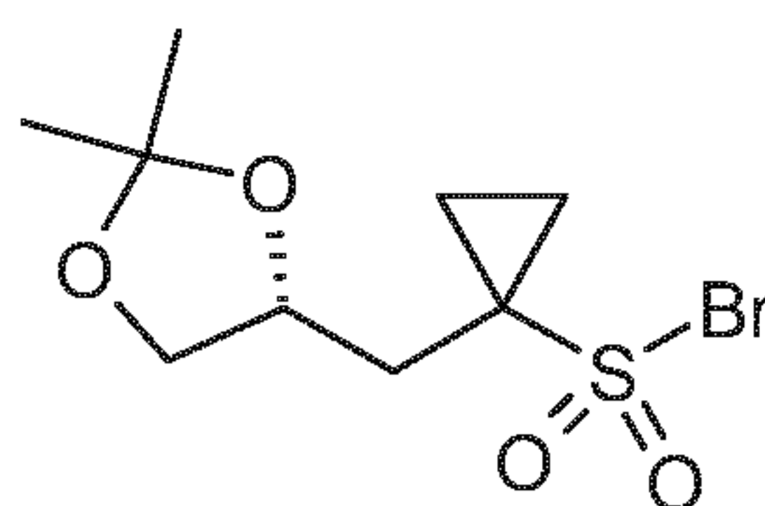
(R)-10-Br
