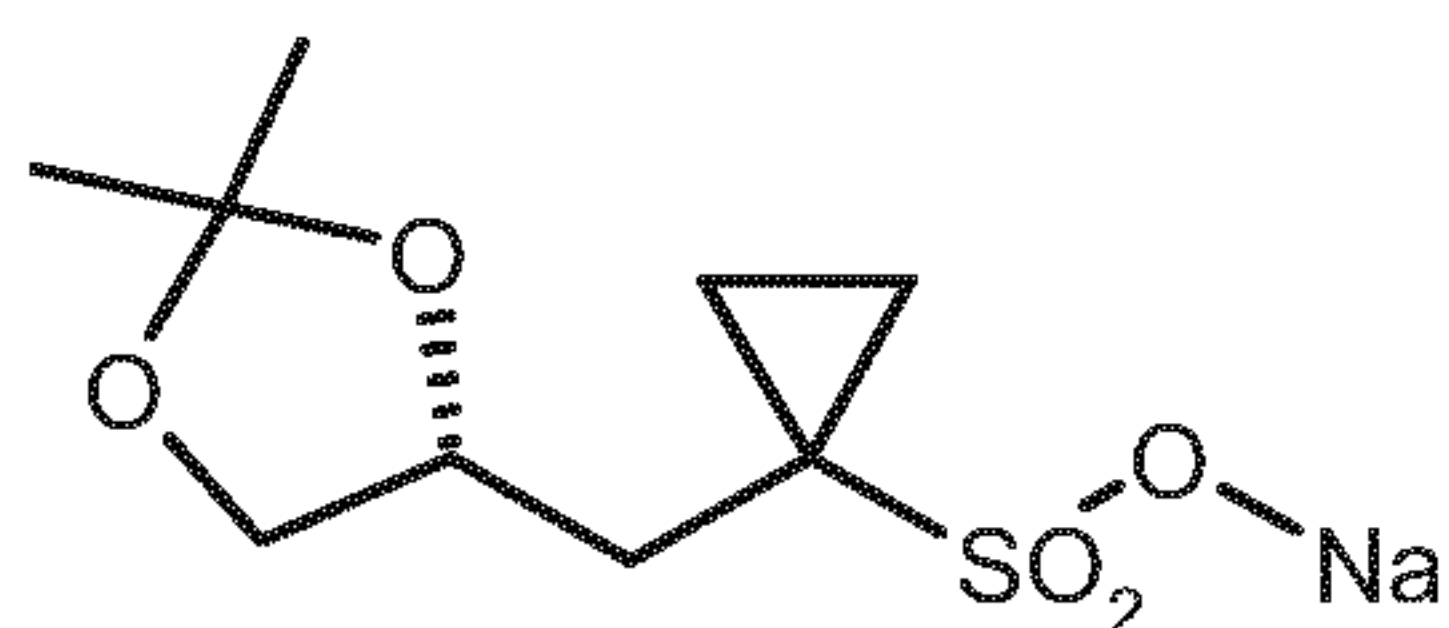
(R)-7
