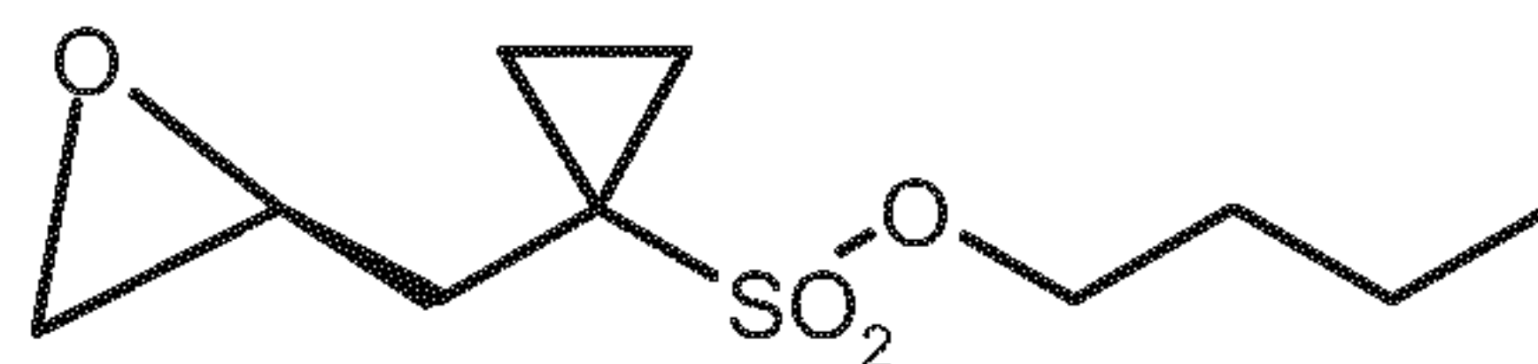
(S)-4
