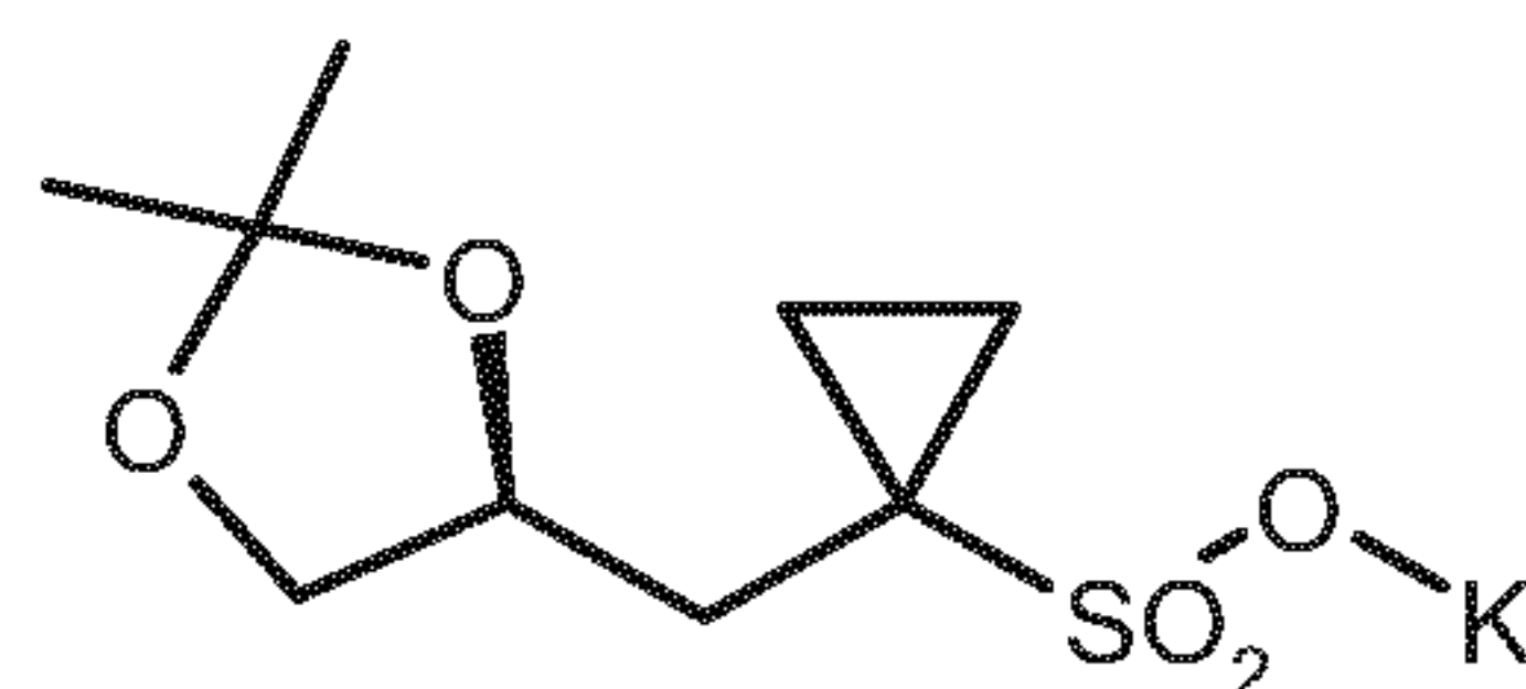
(S)-7'
