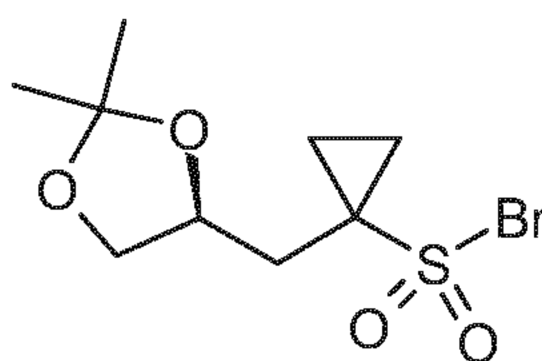
(S)-10-Br
