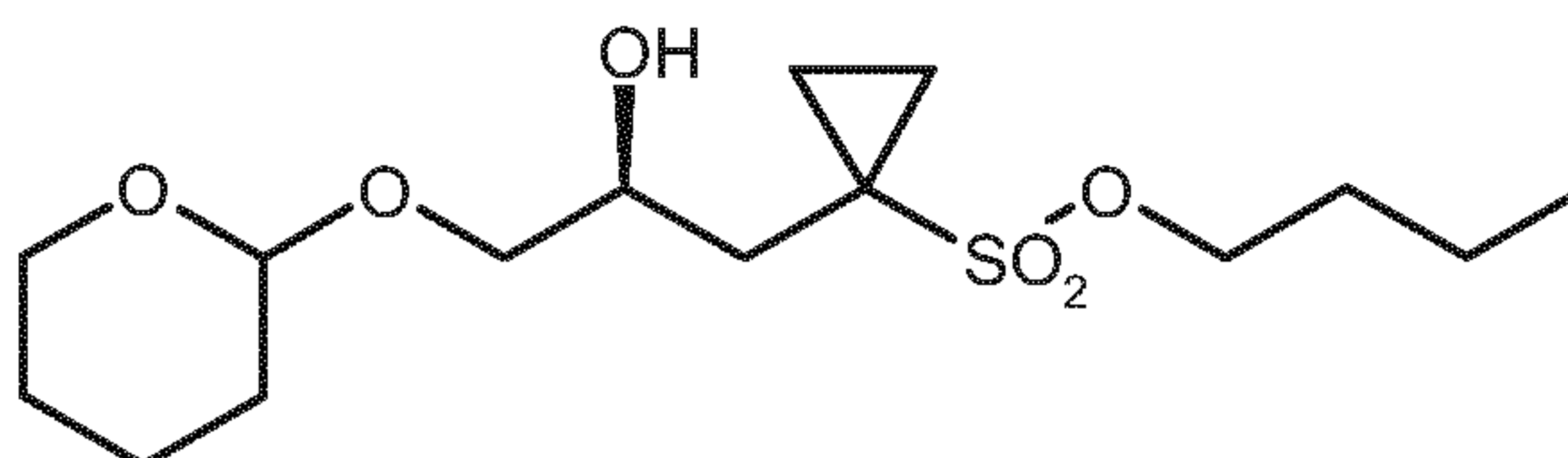
(S)-9b ;
