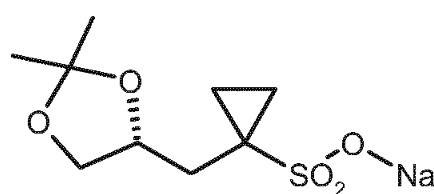
(R)-7
