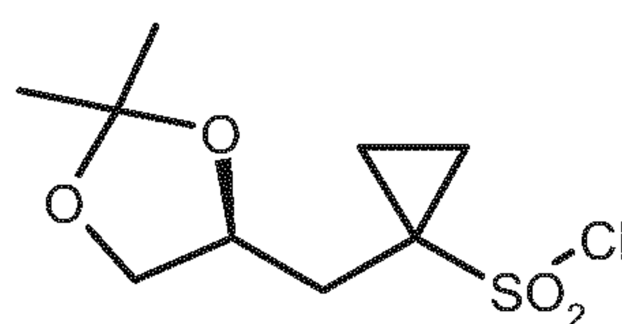
(S)-10
