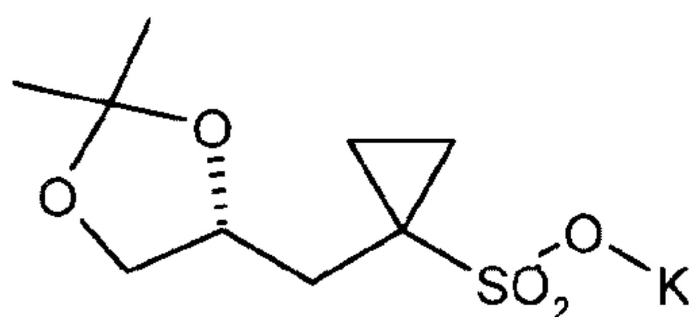
(R)-7' ;
