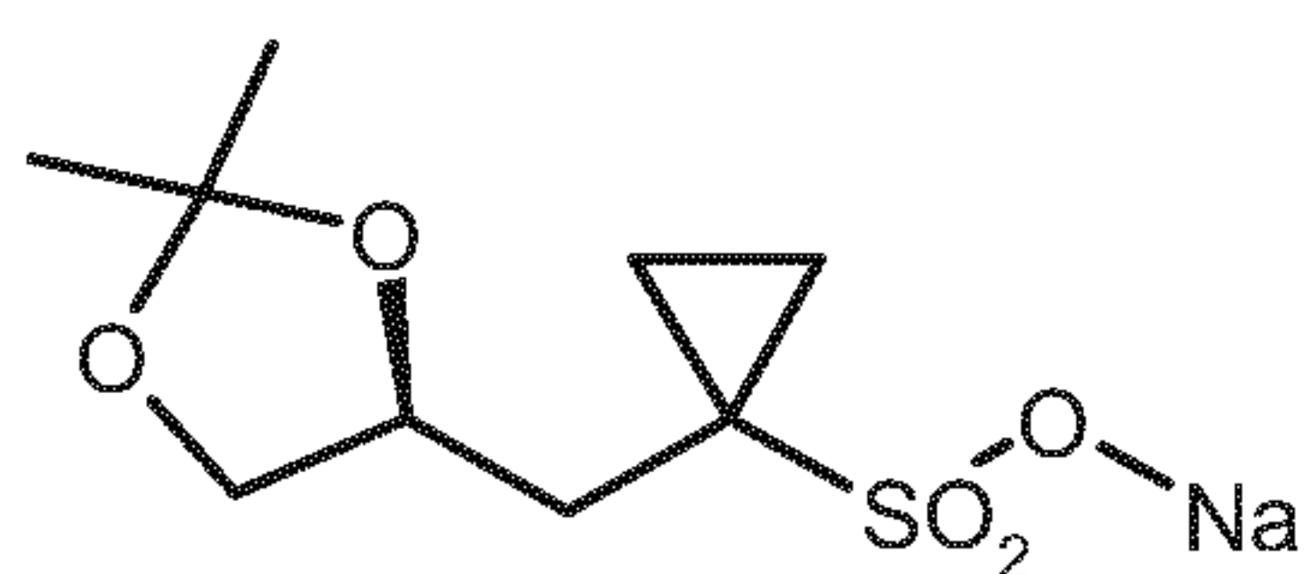
(S)-7
