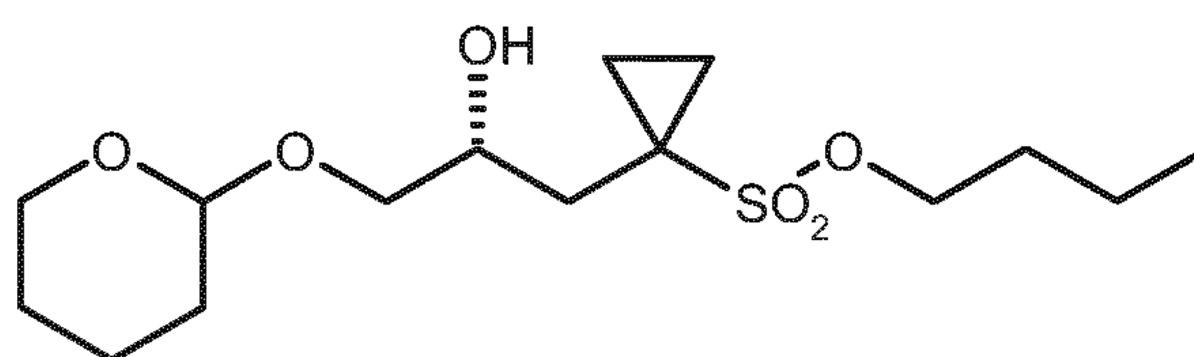
(R)-9b.
