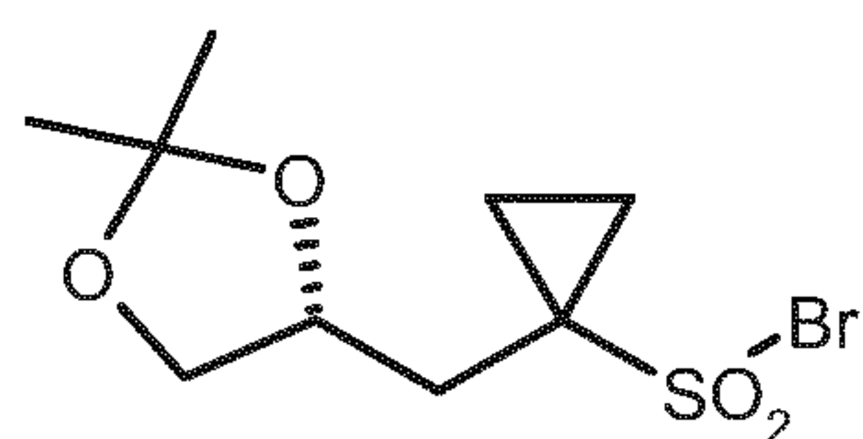
(R)-10-Br
