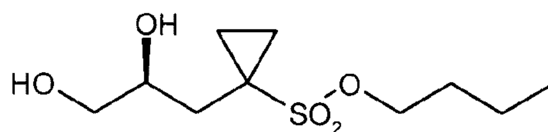
(S)-5
