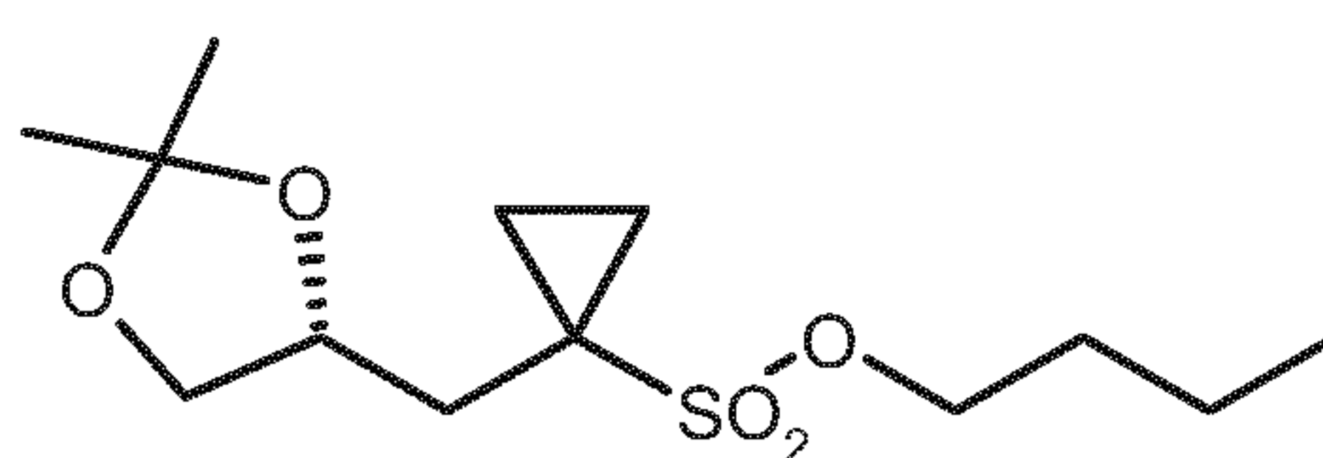
(R)-6
