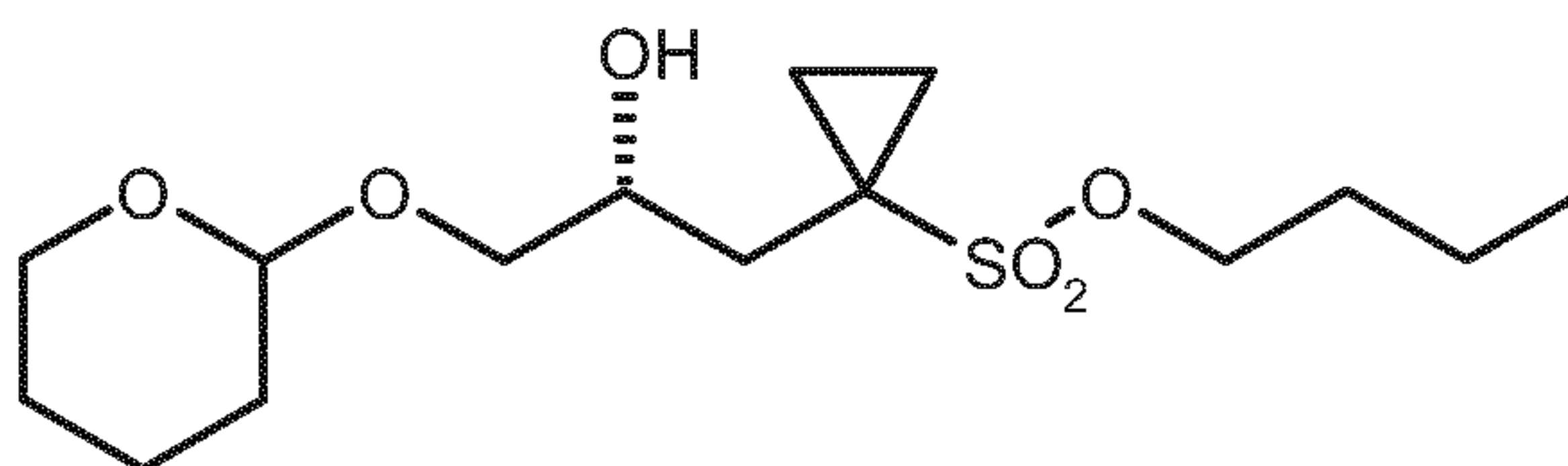
(R)-9b ;
