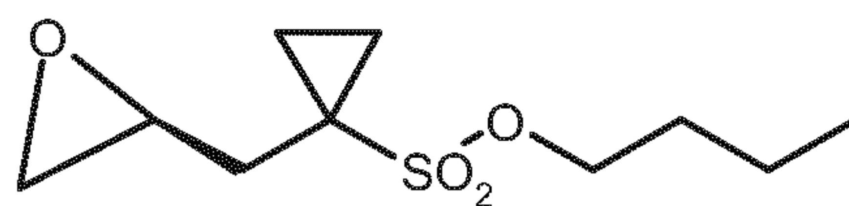
(S)-4
