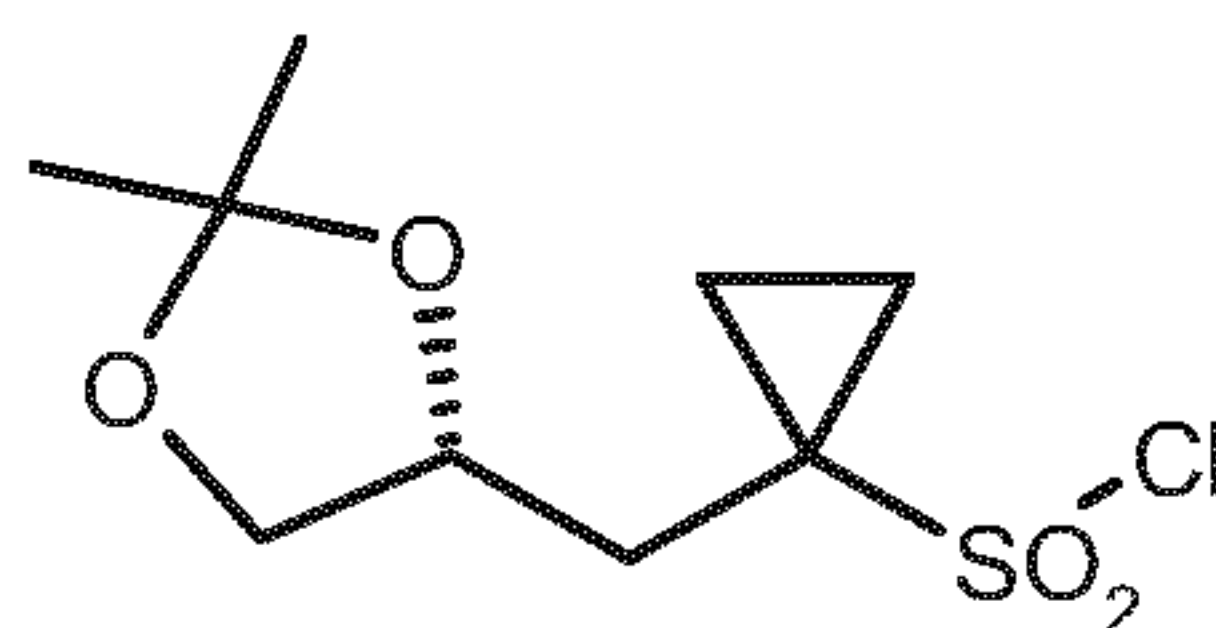
(R)-10
