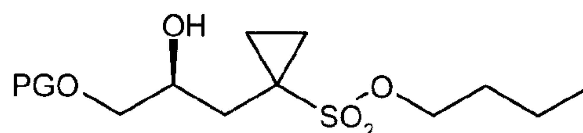
(S)-9 ;
