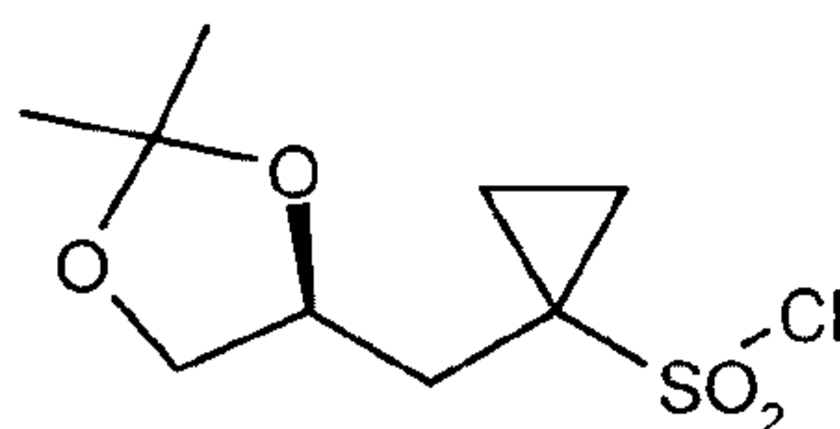
(S)-10
