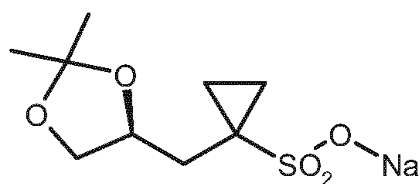
(S)-7
