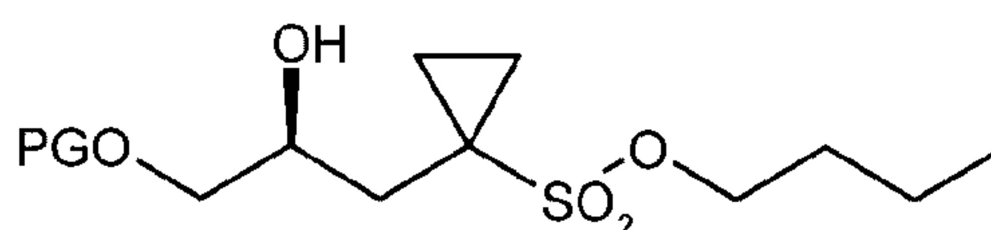
(S)-9 ;
