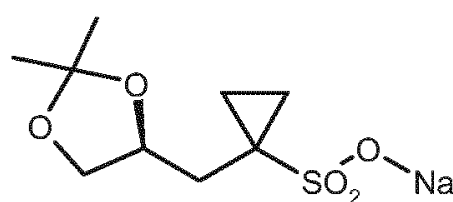
(S)-7
