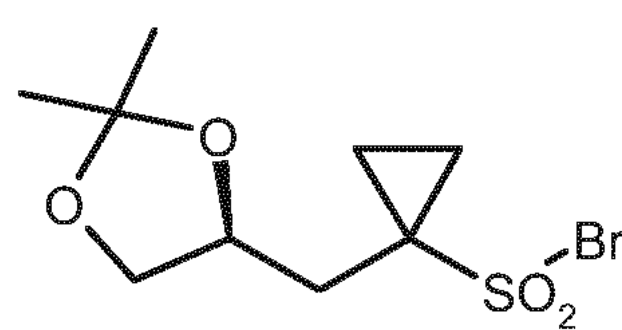
(S)-10-Br
