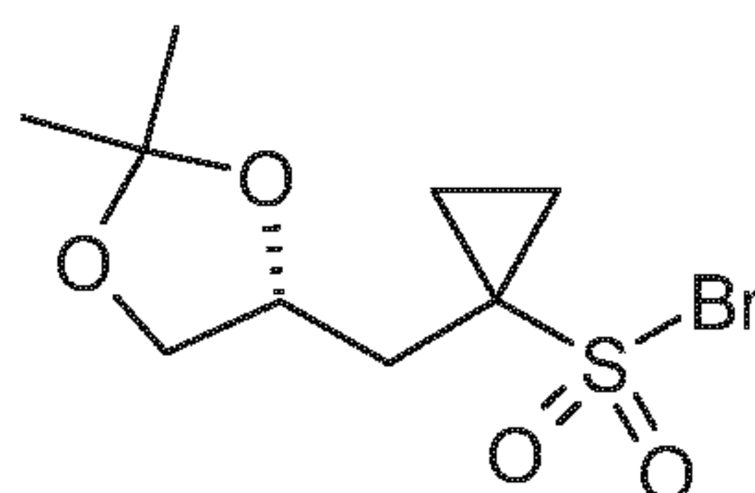
(R)-10-Br
