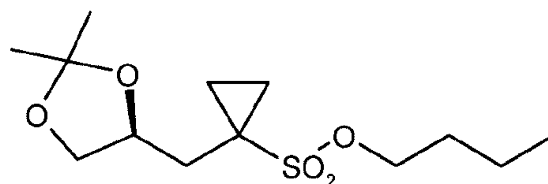
(S)-6 ;
