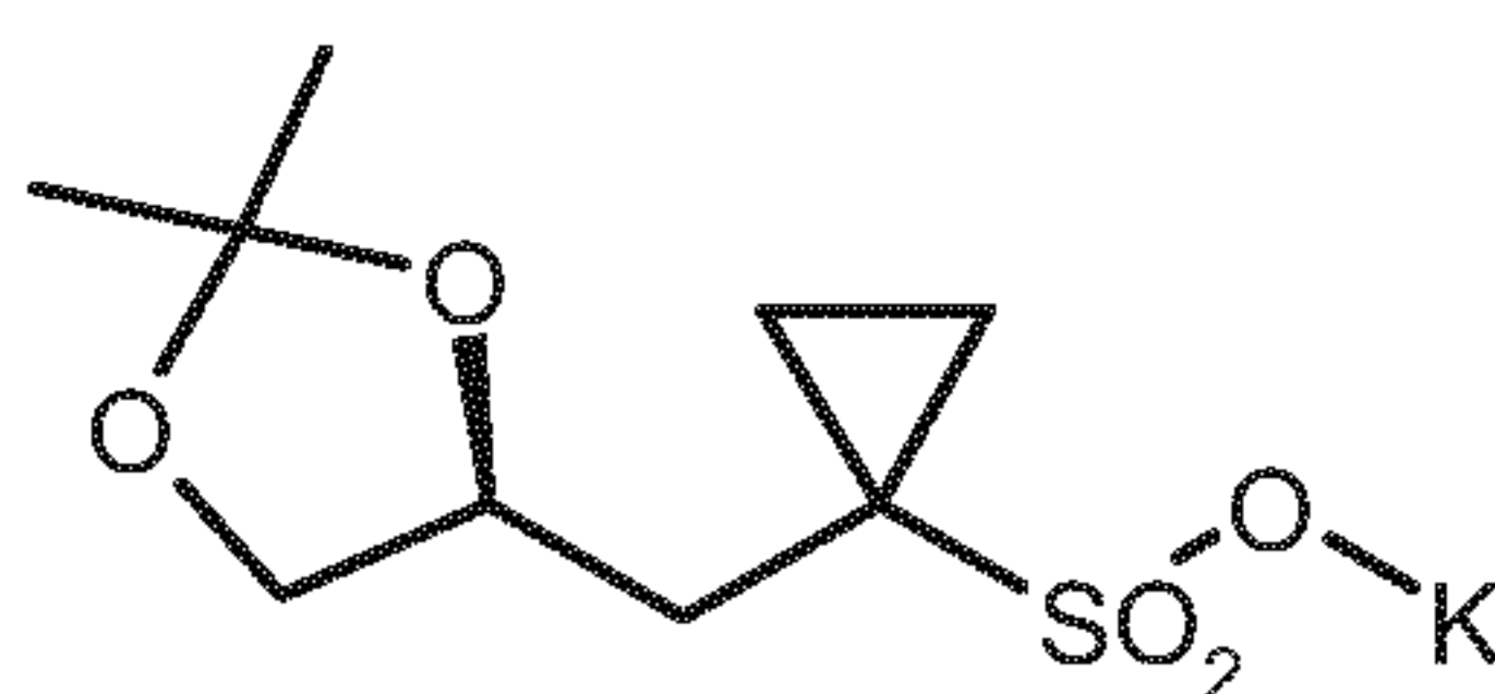
(S)-7'
