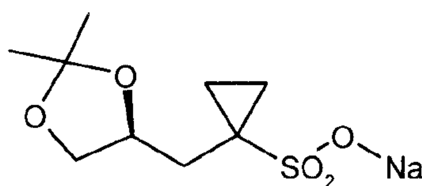
(S)-7
