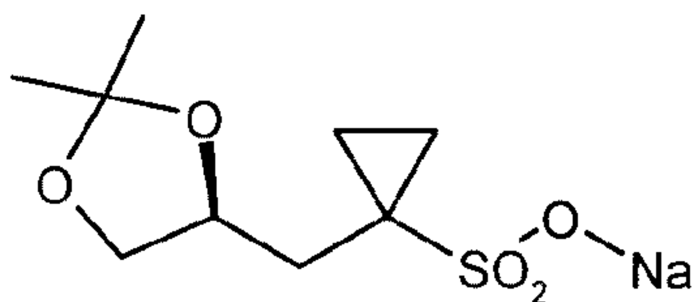
(S)-7
