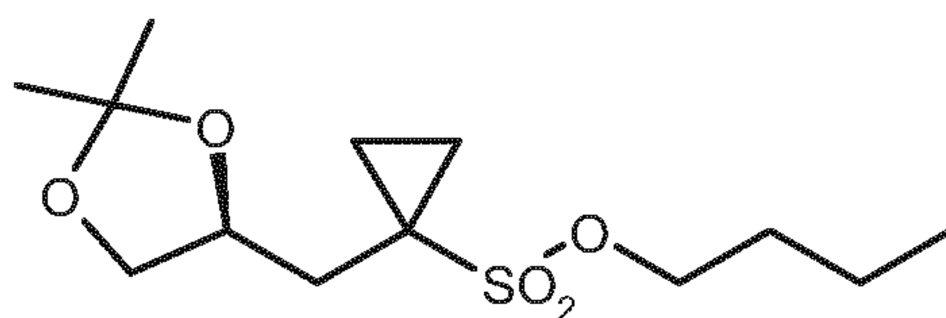
(S)-6
