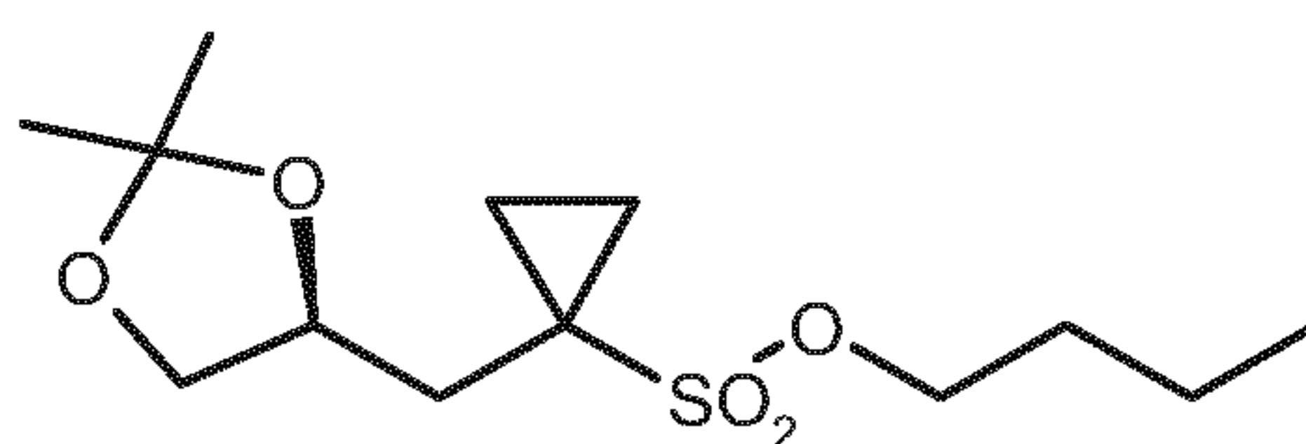
(S)-6
