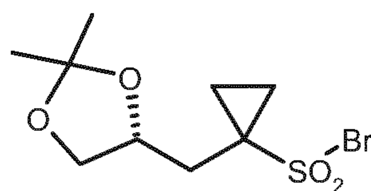
(R)-10-Br
