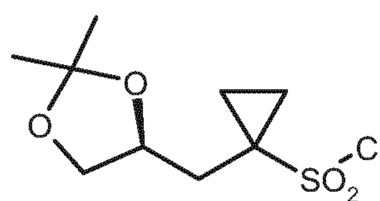
(S)-10
