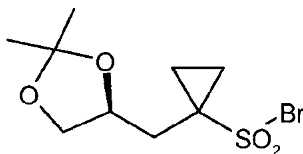
(S)-10-Br
