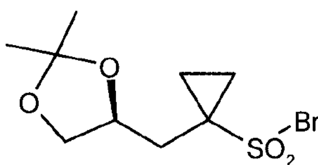
(S)-10-Br
