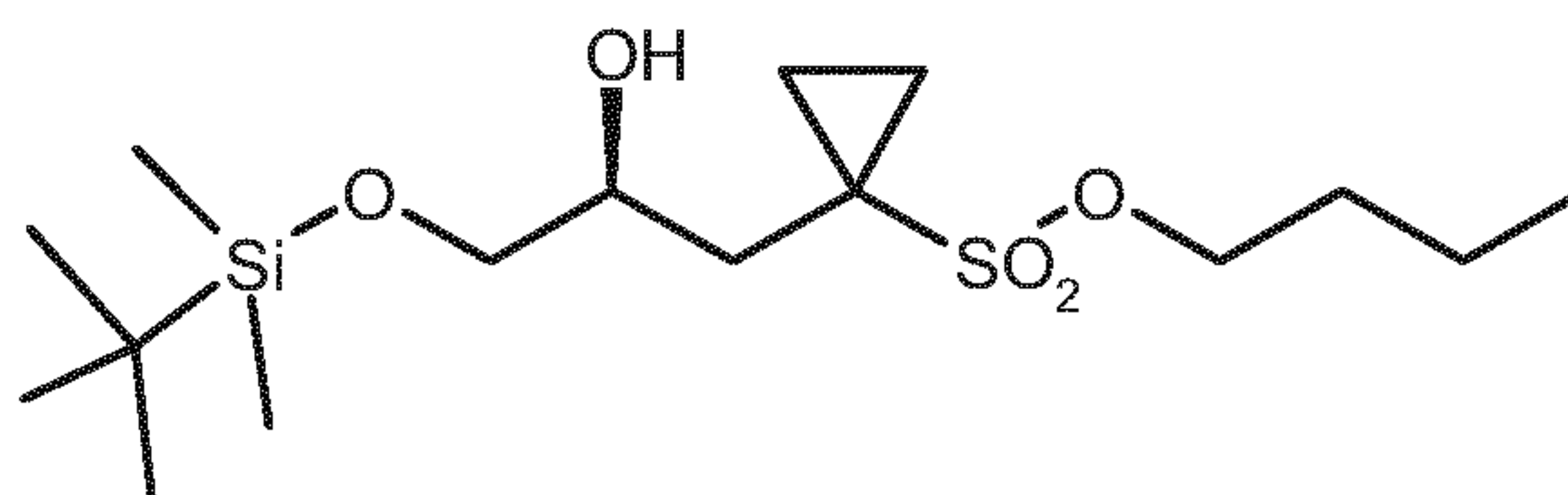
(S)-9a ;
