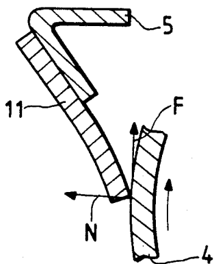
FIG. 6 PRIOR ART
