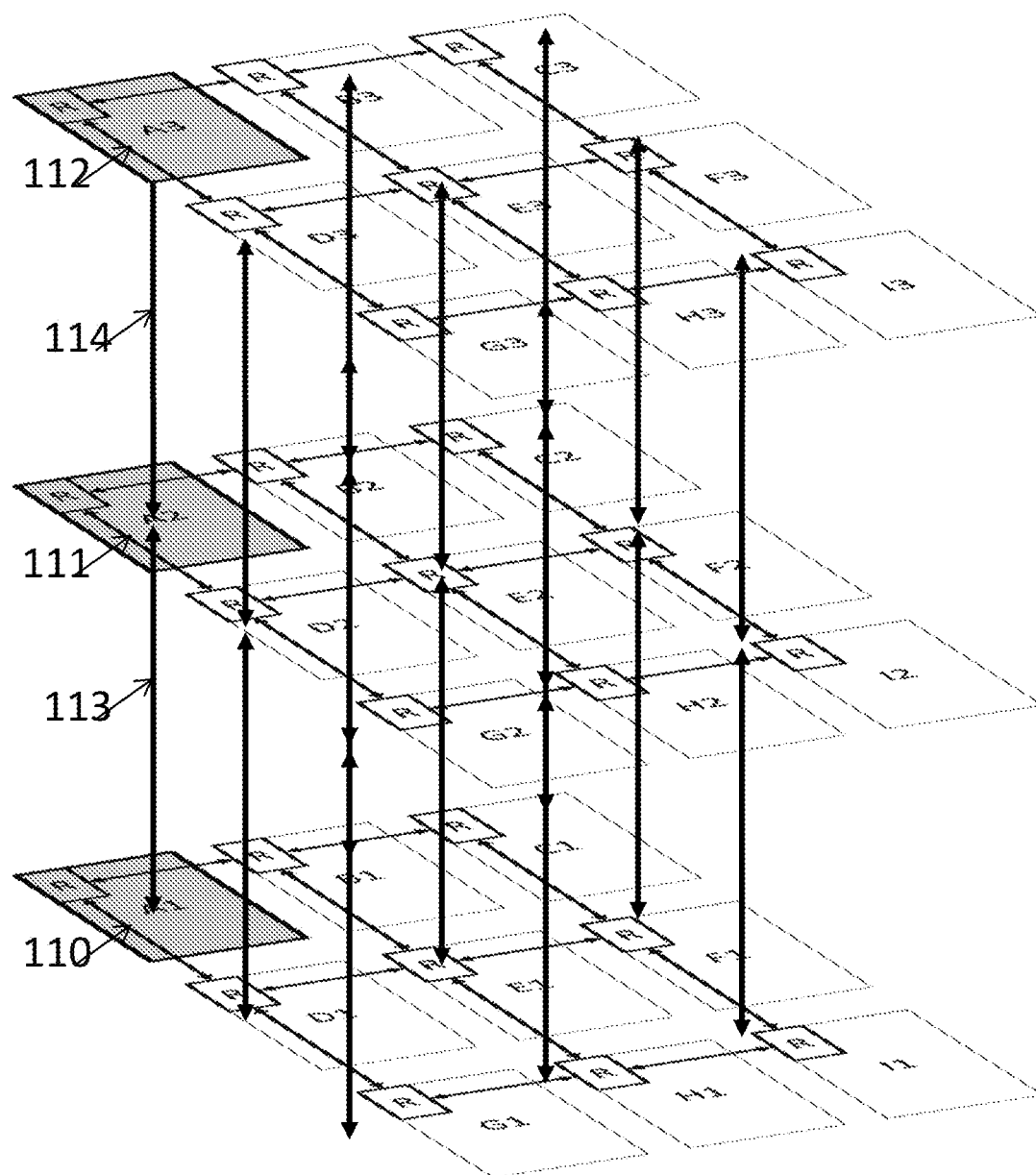
a 3D Mesh NoC topology utilizing router(s){R}
