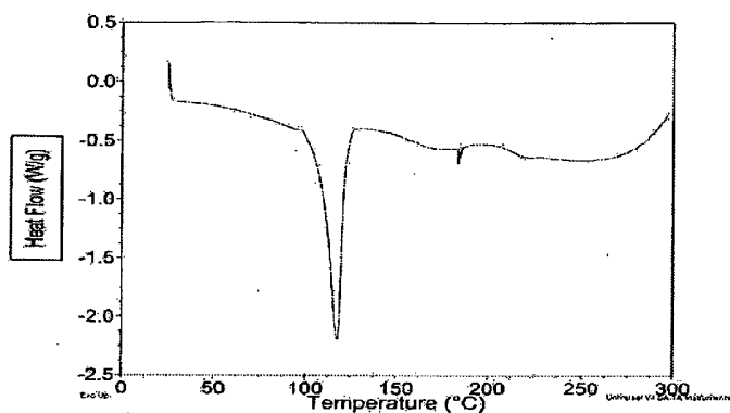
Figure 8: DSC Thermogram N-(2-{2-dimethylaminoethyl-methylamino}-4-methoxy-5- {{4-(1-methylindol-3-yl)pyrimidin-2-yl}amino}phenyl)prop-2-enamide Form D (Monohydrate)
