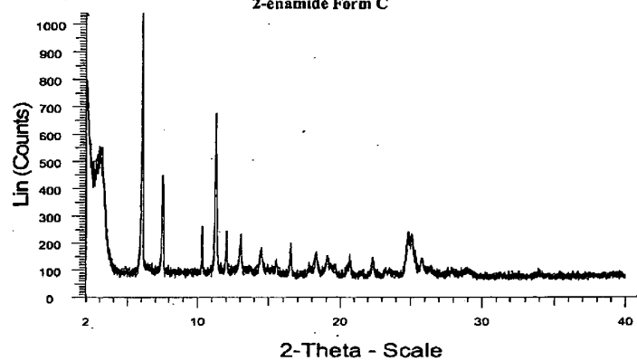
Figure 5: X-Ray Powder Diffraction Pattern N -(2-[2-dimethylaminoethyl-methylamino]-4-methoxy-5-[[4-(1-methylindol-3-yl)pyrimidin-2-yl]amino]phenyl)prop-2-enamide Form C
