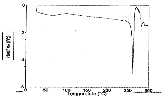
Figure 19: DSC Thermogram N-(2-{2-dimethylaminoethyl-methylamino}-4-methoxy-5- [4-(1-methylindol-3-yl)pyrimidin-2-yl]amino}phenyl)prop-2-enamide Mesylate salt - Form A
