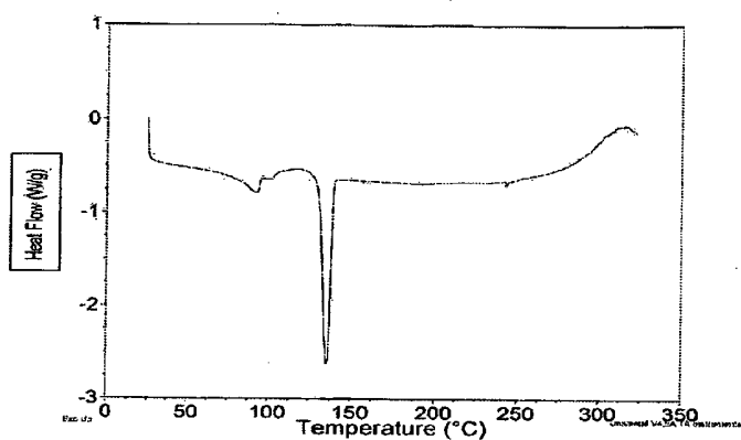
Figure 14: DSC Thermogram N-(2-(2-dimethylaminoethyl-methylamino)-4-methoxy-5- [[4-(1-methylindol-3-yl)pyrimidin-2-yl]amino]phenyl)prop-2-enamide Form F (Hydrated Form)
