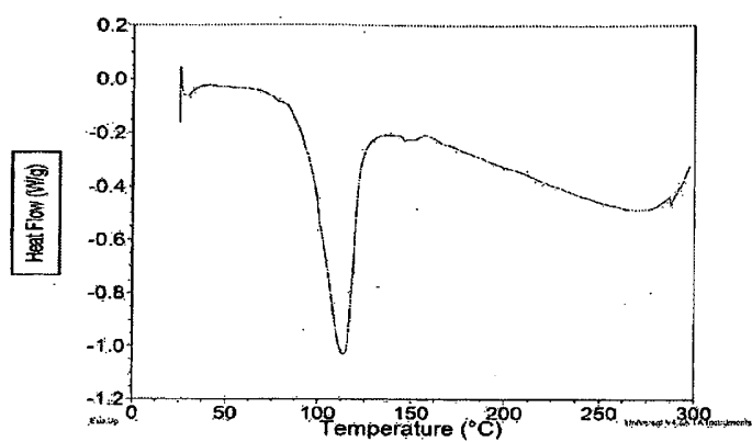
Figure 4: DSC Thermogram N-(2-(2-dimethylaminoethyl-methylamino)-4-methoxy-5- {{4-(1-methylindol-3-yl)pyrimidin-2-yl}amino}phenyl)prop-2-enamide Form B
