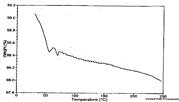
Figure 15: TGA Thermogram N -(2-(2-dimethylaminoethyl-methylamino)-4-methoxy-5-([4-(1-methylindol-3-yl)pyrimidin-2-yl]amino)phenyl)prop-2-enamide Form F (hydrated form)
