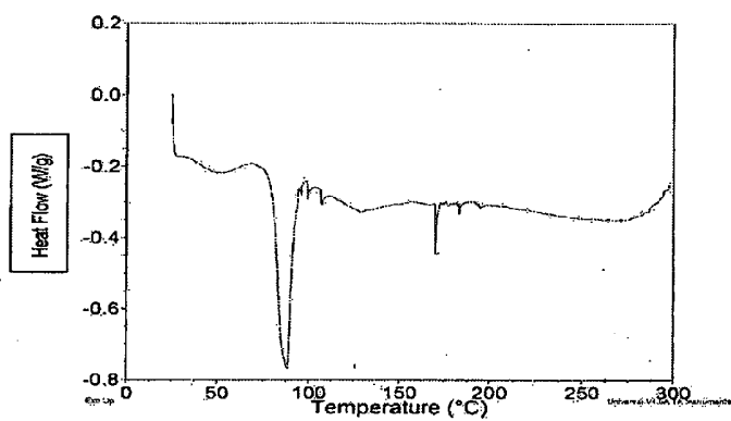
Figure 2: DSC Thermogram N -(2-(2-dimethylaminoethyl-methylamino)-4-methoxy-5- [[4-(1-methylindol-3-yl)pyrimidin-2-yl]amino]phenyl)prop-2-enamide Form A
