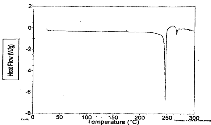
Figure 21: DSC Thermogram N-(2-{2-dimethylaminoethyl-methylamino}-4-methoxy-5- [4-(1-methylindol-3-yl)pyrimidin-2-yl]amino}phenyl)prop-2-enamide Mesylate salt - Form B
