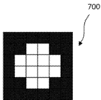
EXAMPLE INPUT KERNEL FOR EROSION IMAGE PROCESSING
