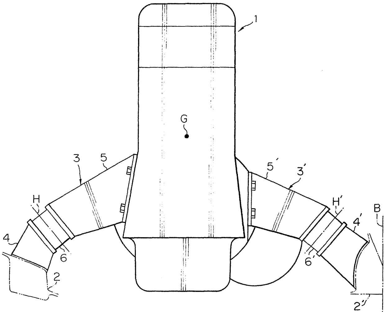
FIG. 1 PRIOR ART
