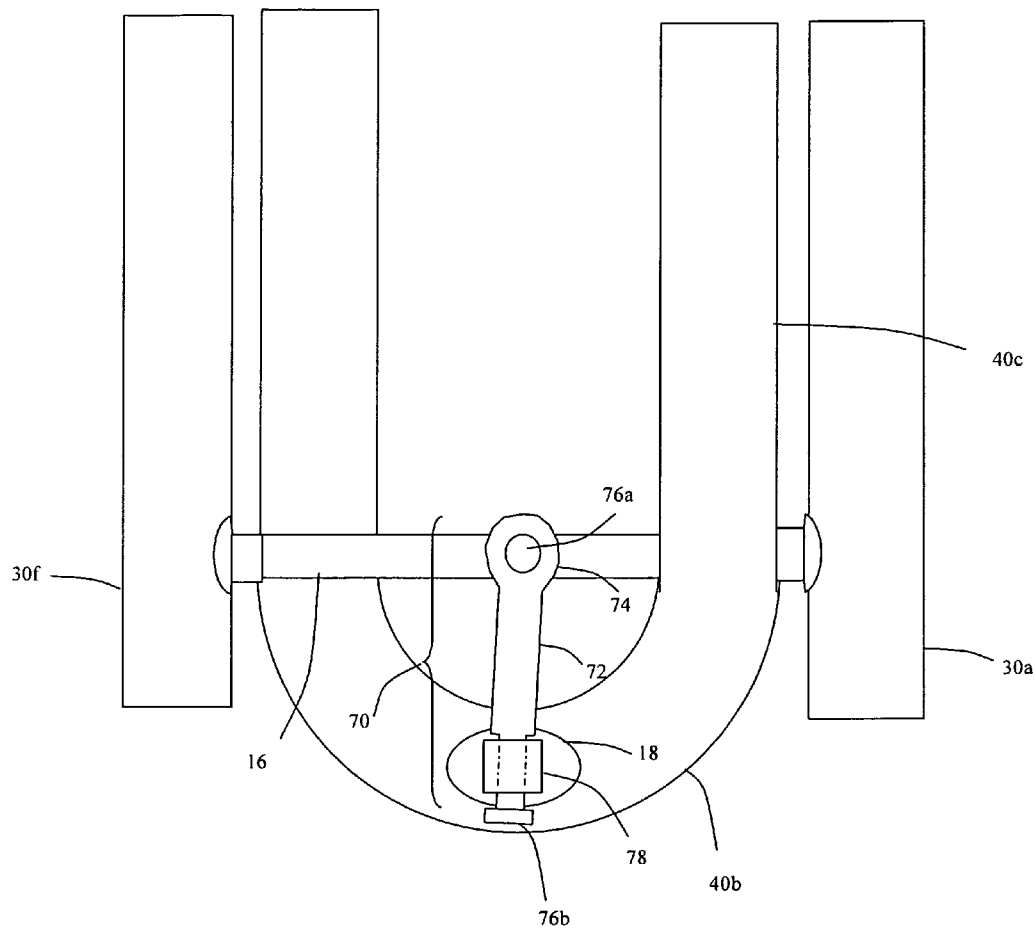
Detail 1D
