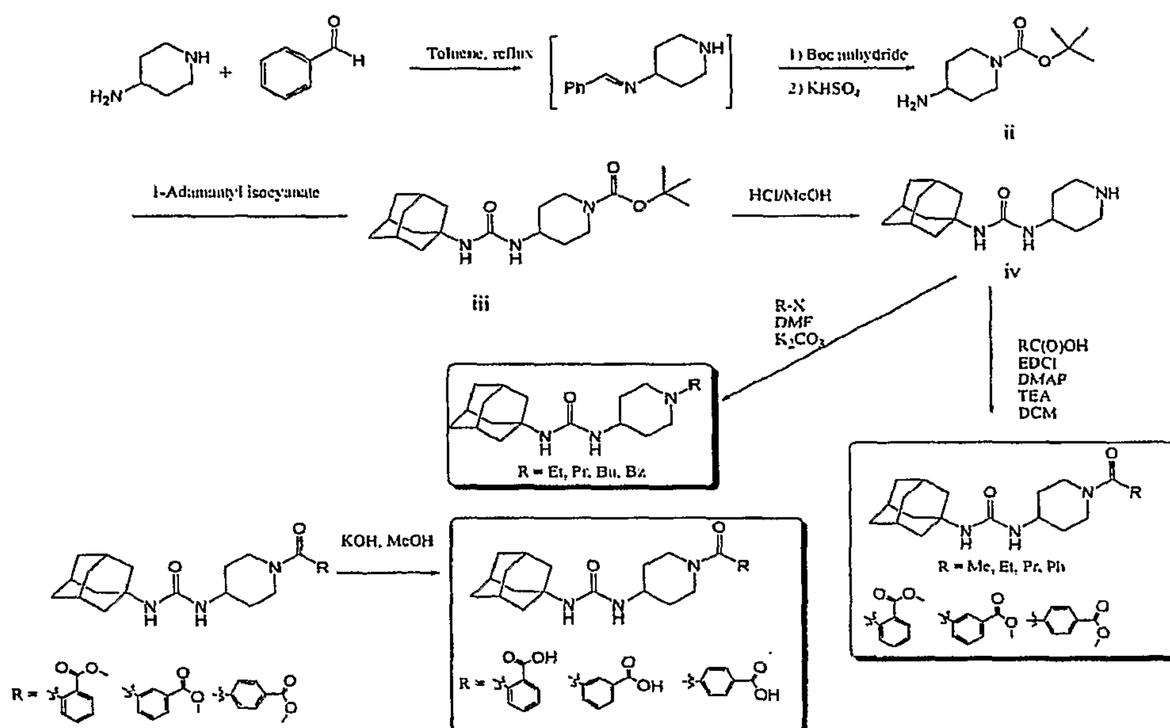
Scheme 1: Synthesis of N-(1-benzoylpiperidin-4-yl)-N'-(adamant-1-yl)ureas.
