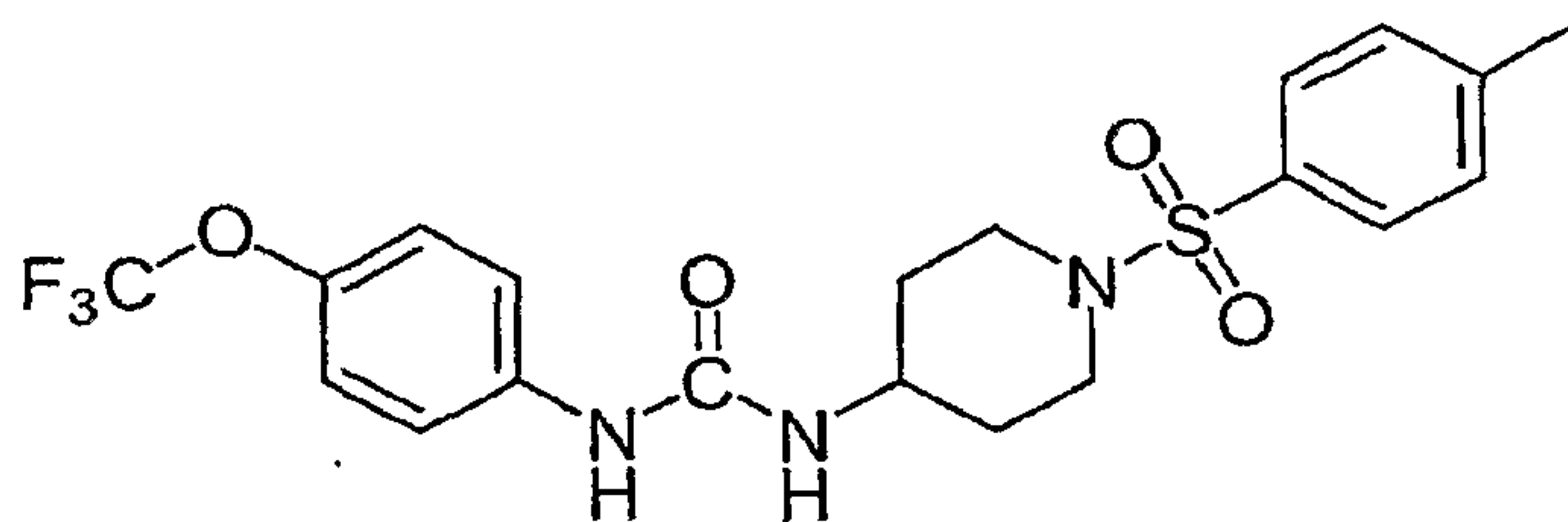
1-[1-(Toluene-4-sulfonyl)-piperidin-4-yl]-3-(4-trifluoromethoxy-phenyl)-urea (1711)
