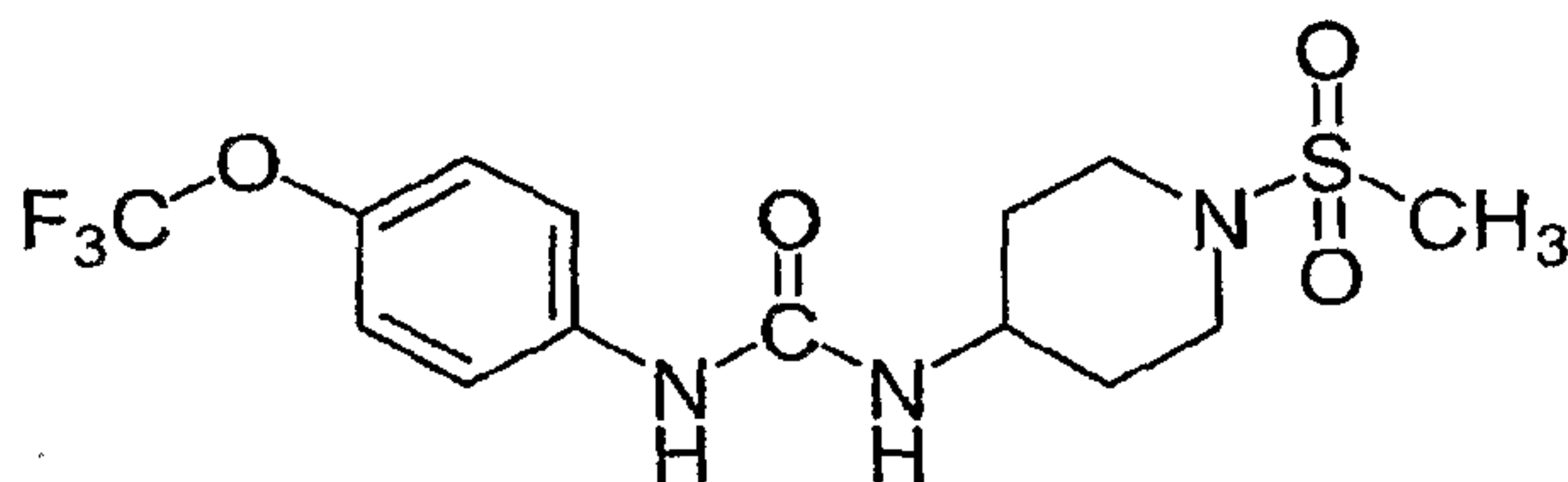
1-(1-Methanesulfonyl-piperidin-4-yl)-3-(4-trifluoromethoxy-phenyl)-urea (1709)
