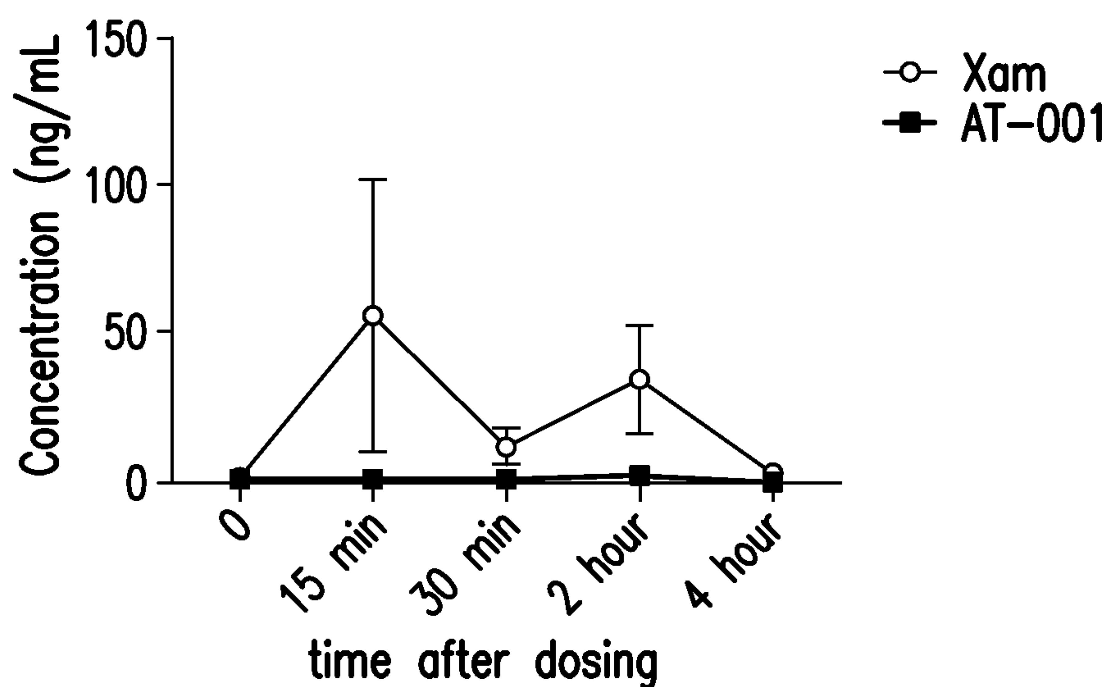
Xamoterol and AT-001 level after dosing AT-001 (Oral)
