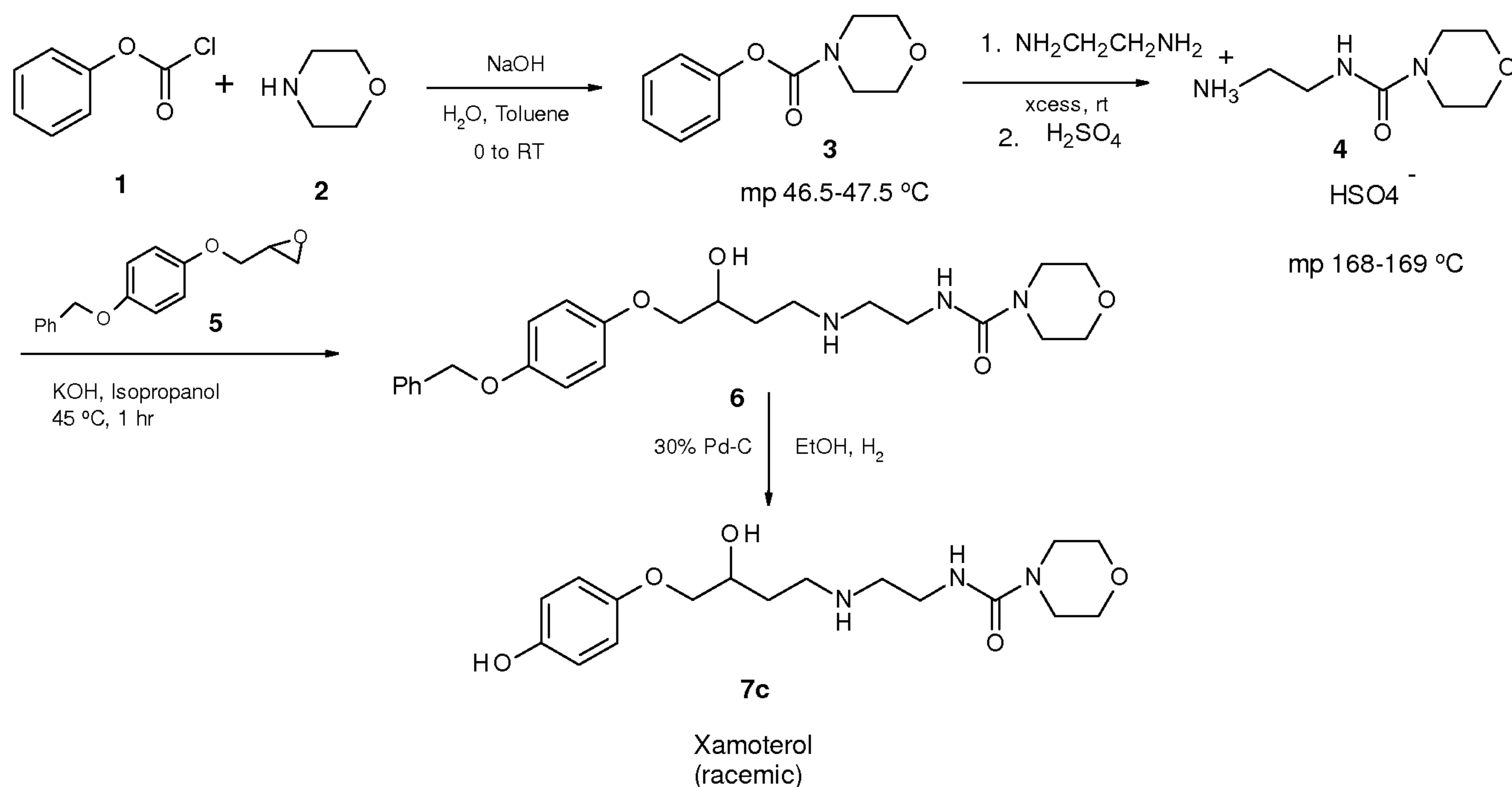
Scheme 2. Synthesis of racemic Xamoterol:
