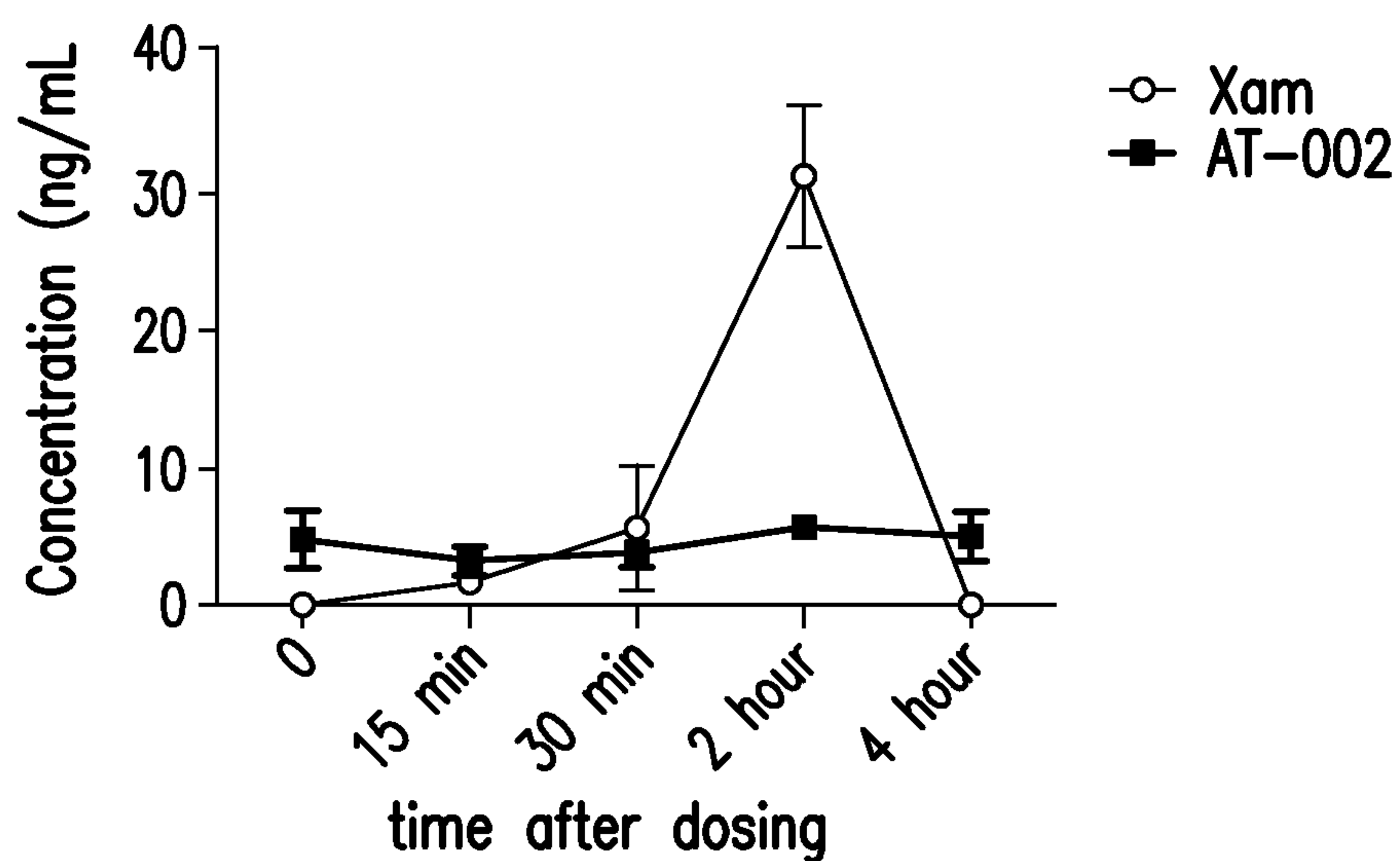
Xamoterol and AT-002 level after dosing AT-002 (Oral)
