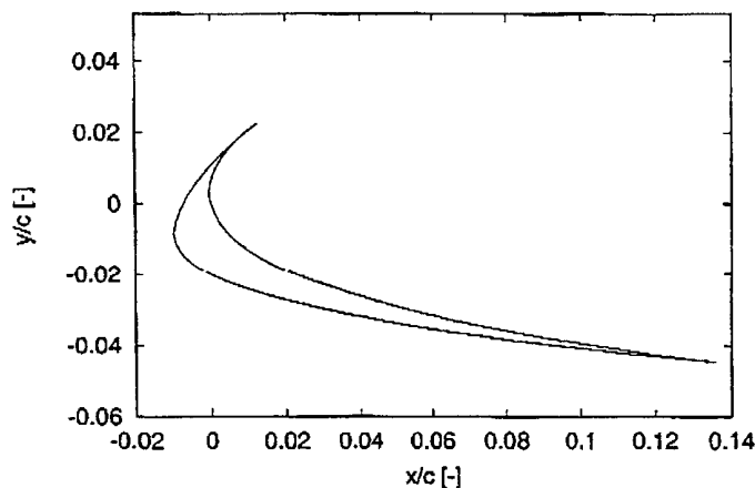
Device for modifying stall characteristics for NACA 63-415
