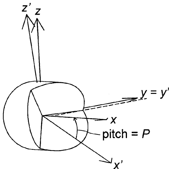
PERSPECTIVE VIEW
