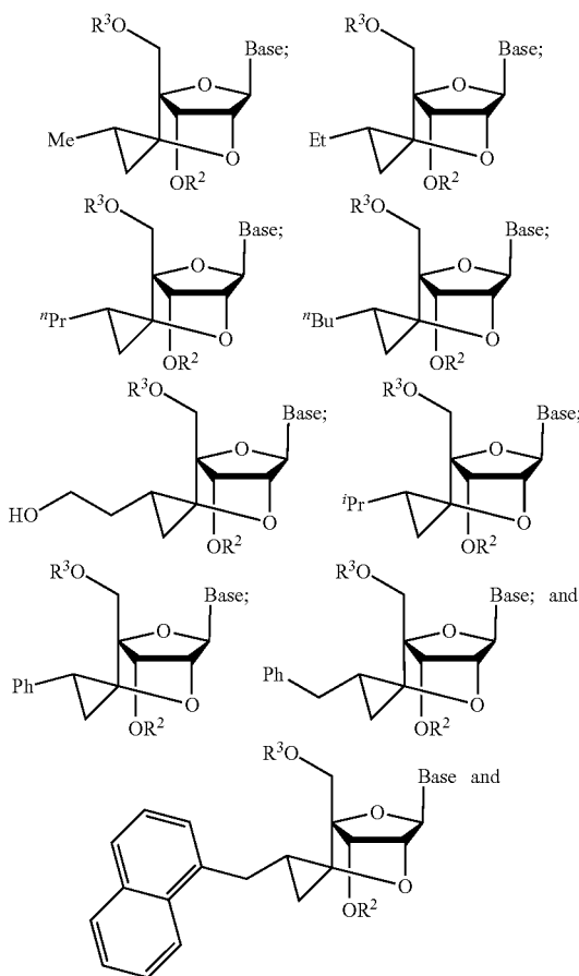
[Chemical 8]
