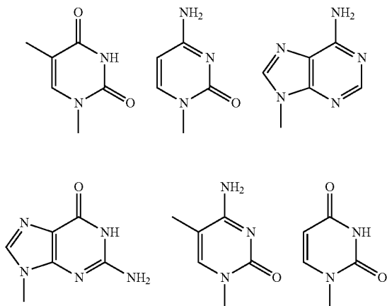
[Chemical 6]
