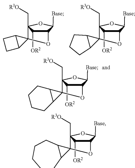
[Chemical 8]
