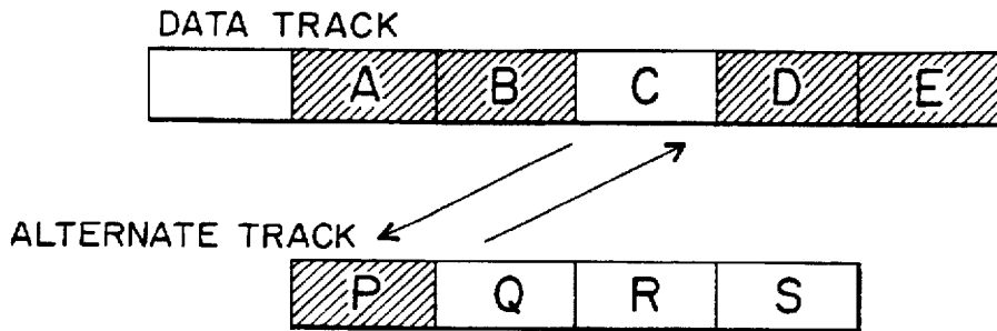
FIG. 8 (PRIOR ART)
