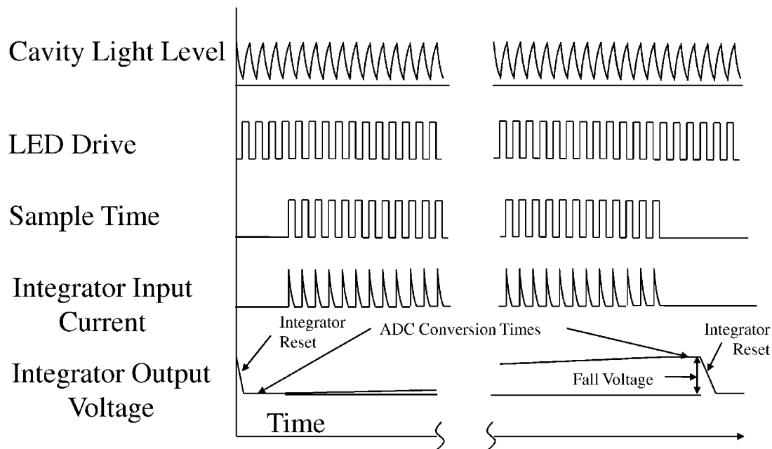
Example Fall Time Measurement Interval
