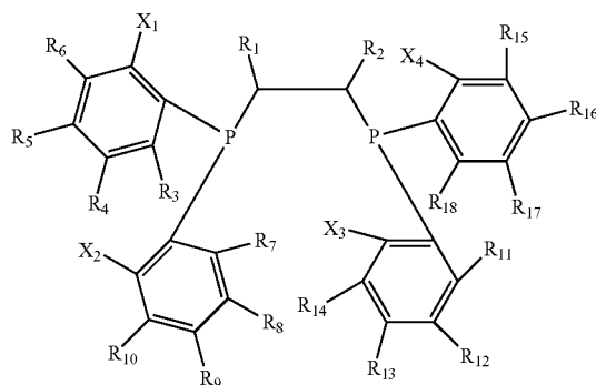
ChemistryFigure 1
