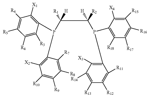
ChemistryFigure 3
