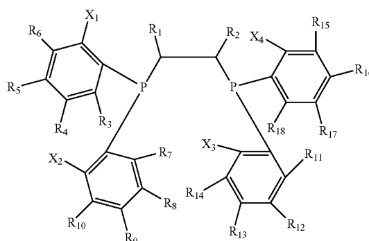
[Chemical Formula 1]
