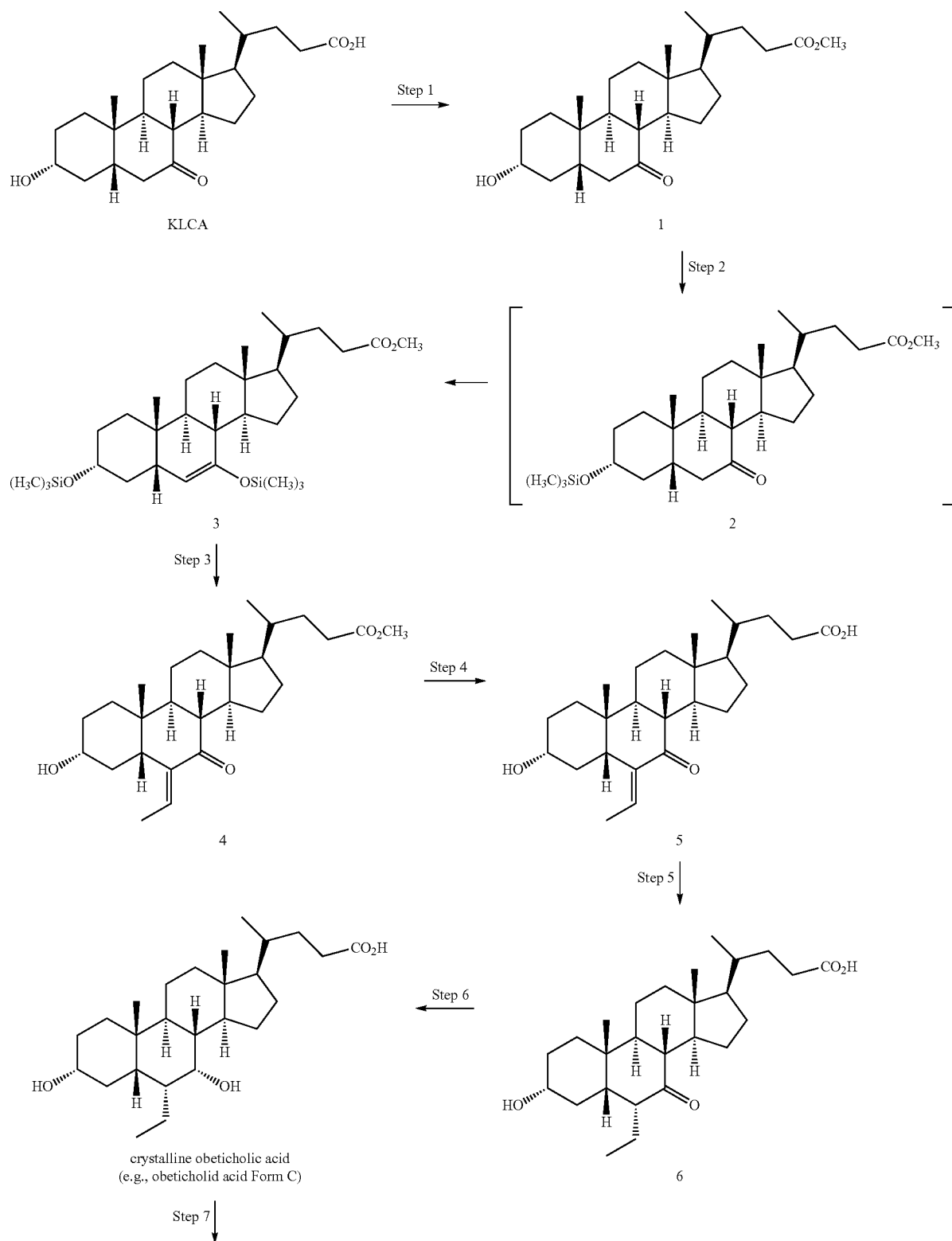
Scheme 11
