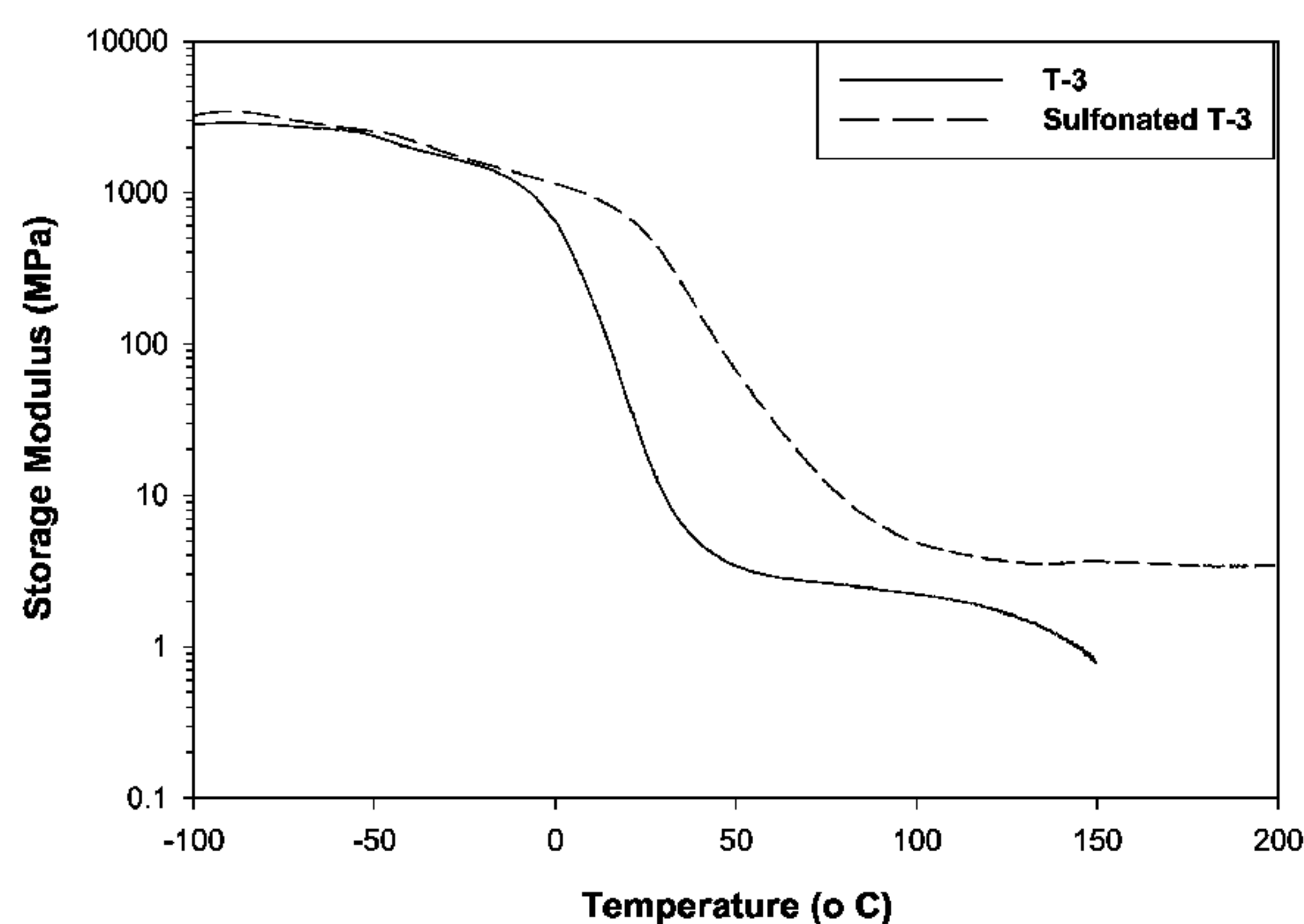
Polymer T-3 Before and After Sulfonation
