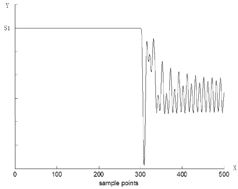
Forward fault
