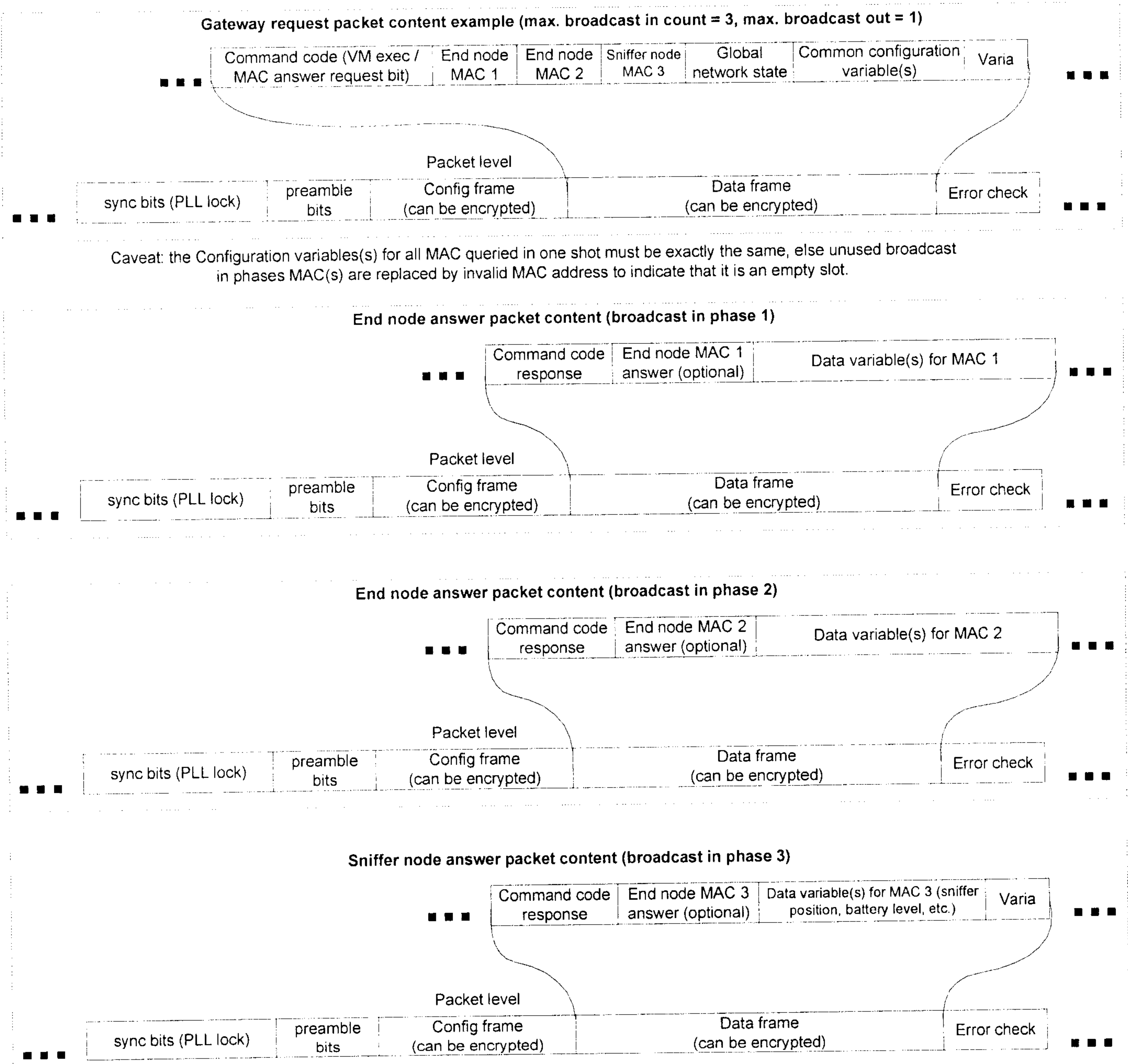
FIGURE 16 - ASYMMETRIC SNIFFER ENABLED NETWORK IMPLEMENTATION – PACKET CODEC
