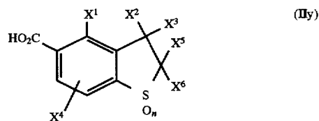
Production scheme 7
