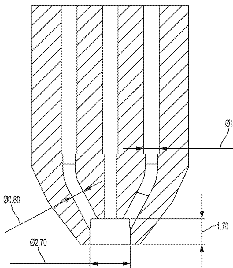
SECTION B-B FIG. 1F
