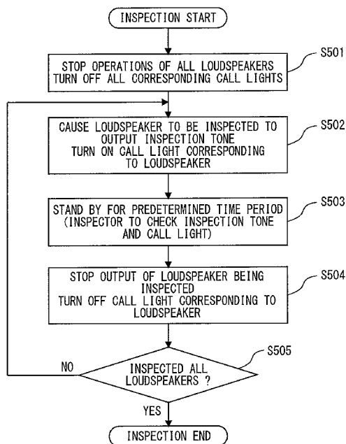
LOUDSPEAKER INSPECTING METHOD 500
