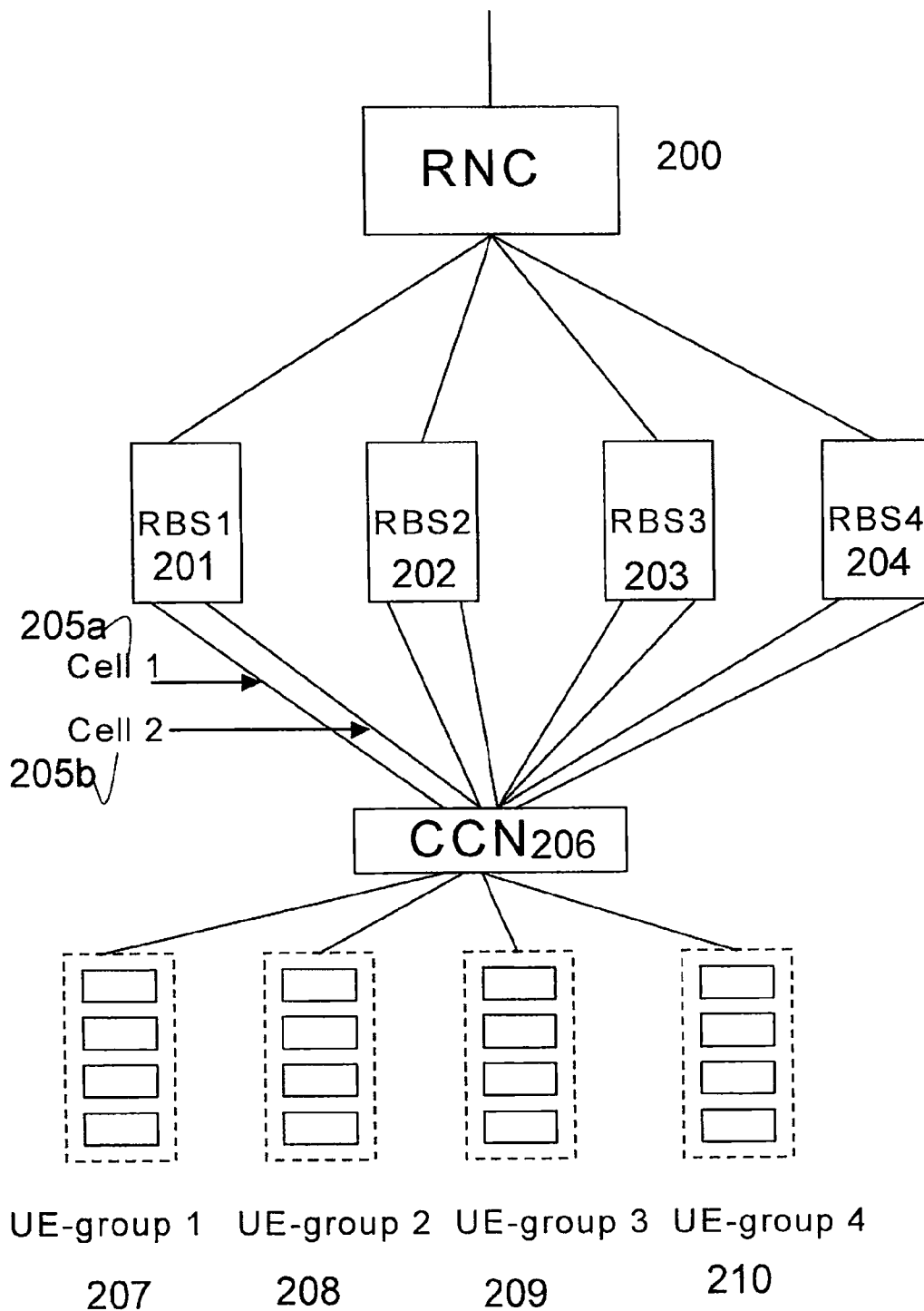
Fig. 2 Physical layout
