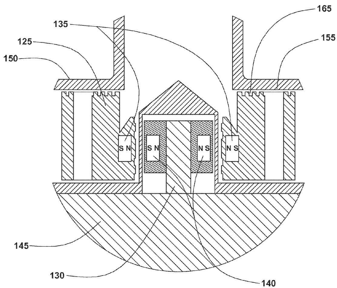
FIG. 13 (DETAIL D)
