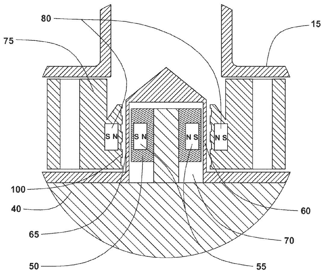
FIG 4 (DETAIL C)
