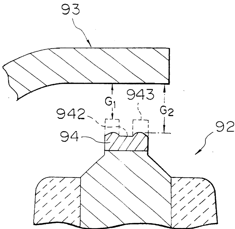
FIG. 16 (PRIOR ART)
