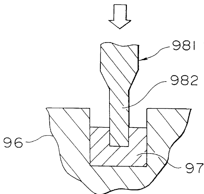
FIG. 18 (PRIOR ART)
