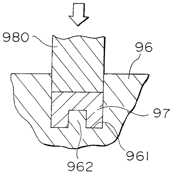
FIG. 17 (PRIOR ART)
