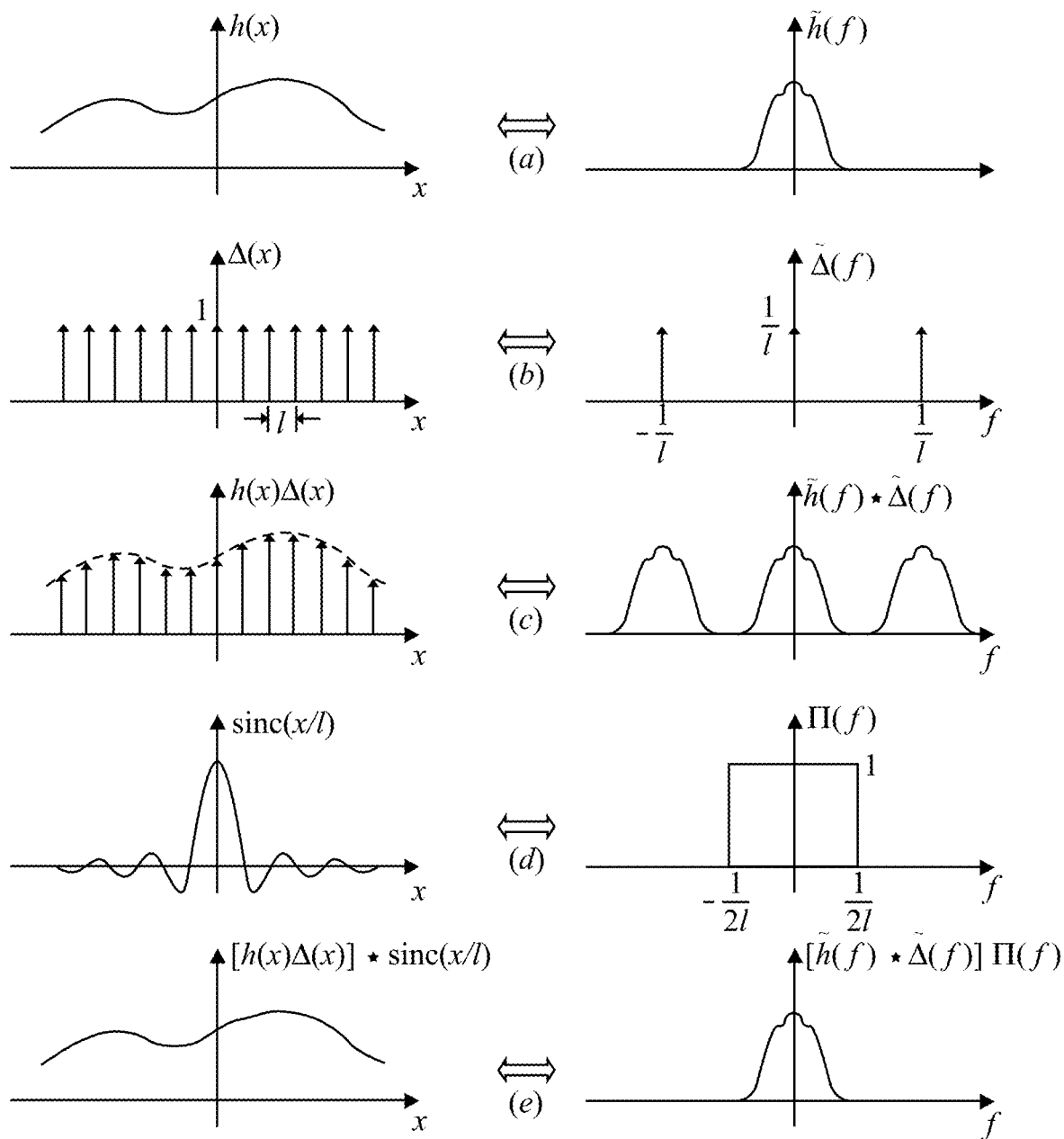
FIG. 3 (PRIOR ART)
