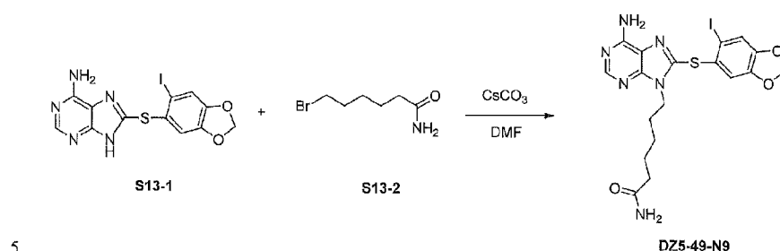
Scheme 13. Synthesis of DZ5-49-N9.
