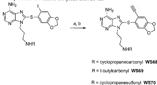
Scheme 12. Synthesis of S-linked acetylene derivatives.
