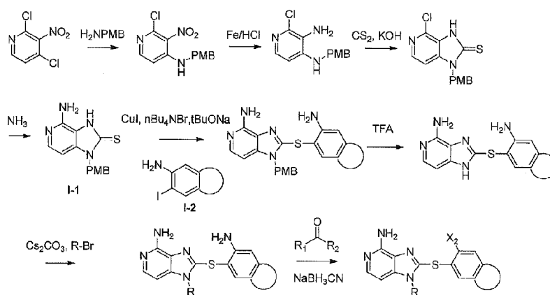
Scheme 3. Synthesis of Pyridine Derivatives (The definitions of R and X 2 as an amino group in this scheme are described above.)
