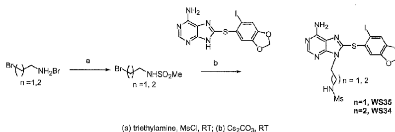
Scheme 4. Synthesis of WS34 and WS35
