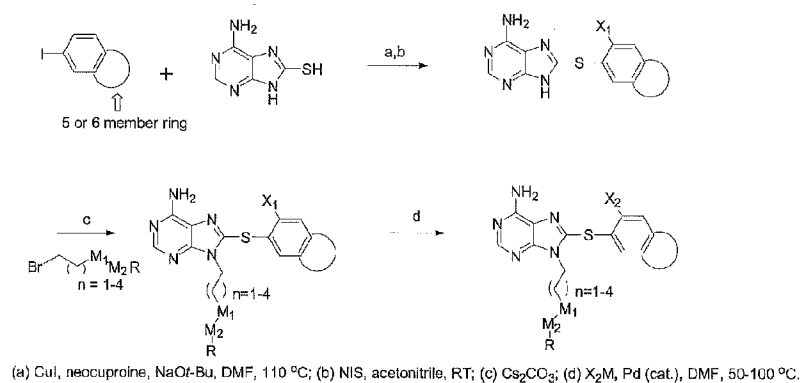
Scheme 1. Synthesis of S-linker Adenine Derivatives
