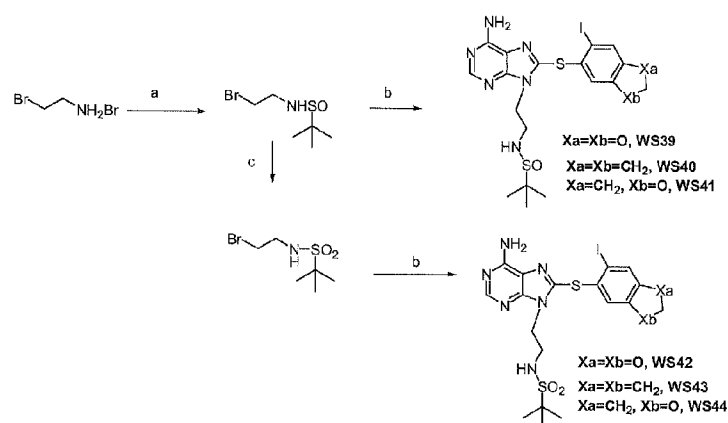
Scheme 7. Synthesis of Compounds from WS39 through WS44
