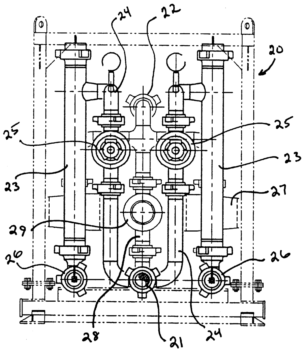
INLET ELEVATION
