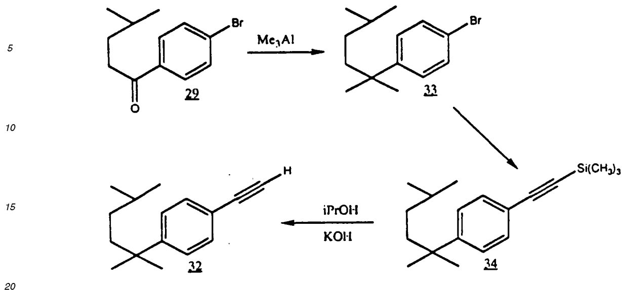
Reaction Scheme 6
