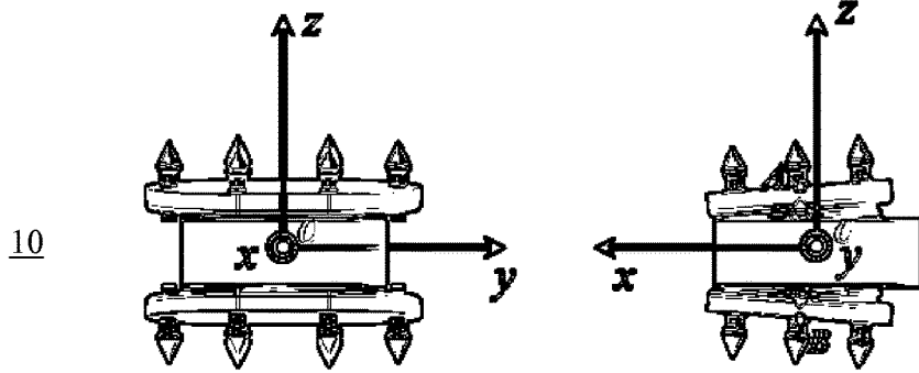
Figure 4Ci: Front View
