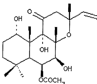
Structure of Isoforskolin
