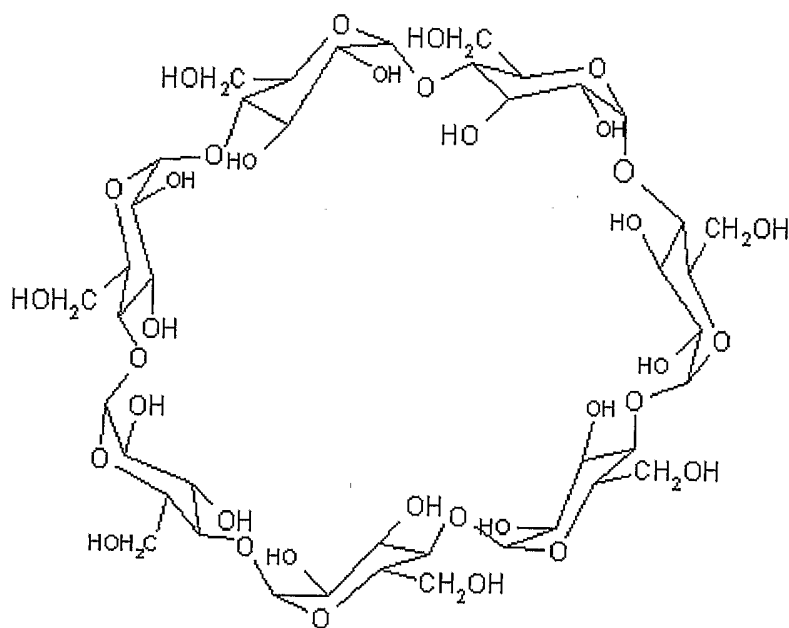
Structure of Beta-cyclodextrin
