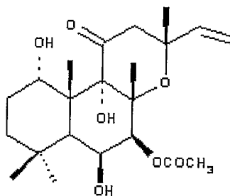
Structure of Forskolin
