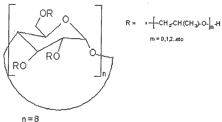
Structure of HPGCD
