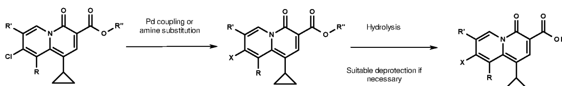
Scheme 1: Preparation of 2-pyridones from scaffolds in 2 or 3 steps.
