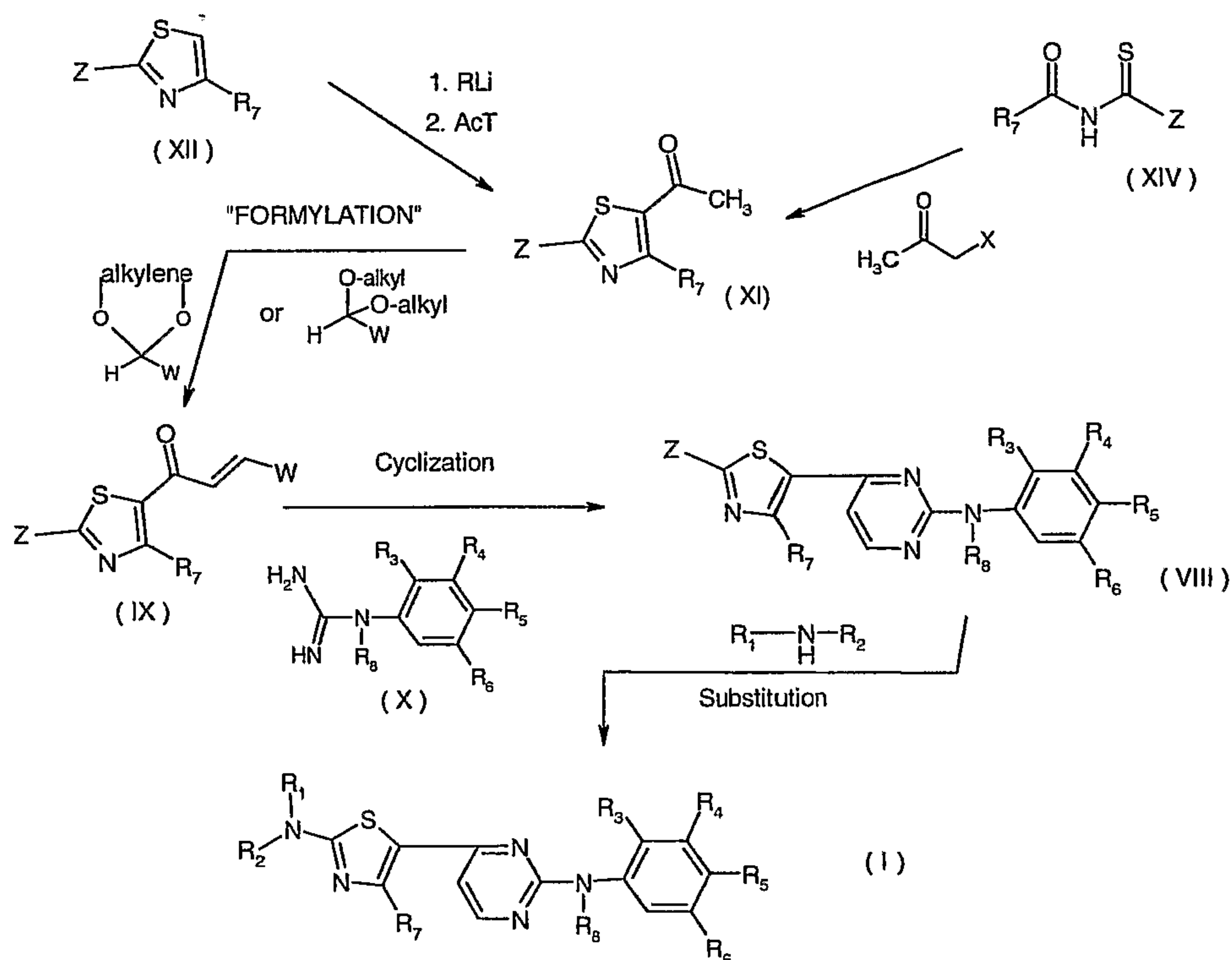
Scheme 2: Route via an acetylthiazole :
